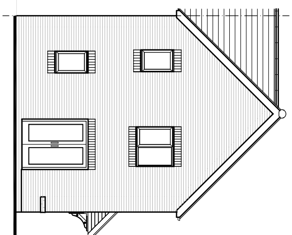
REAR ELEVATION
