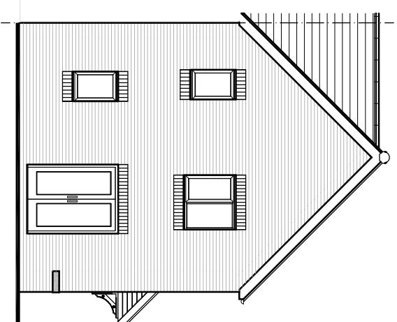
REAR ELEVATION
