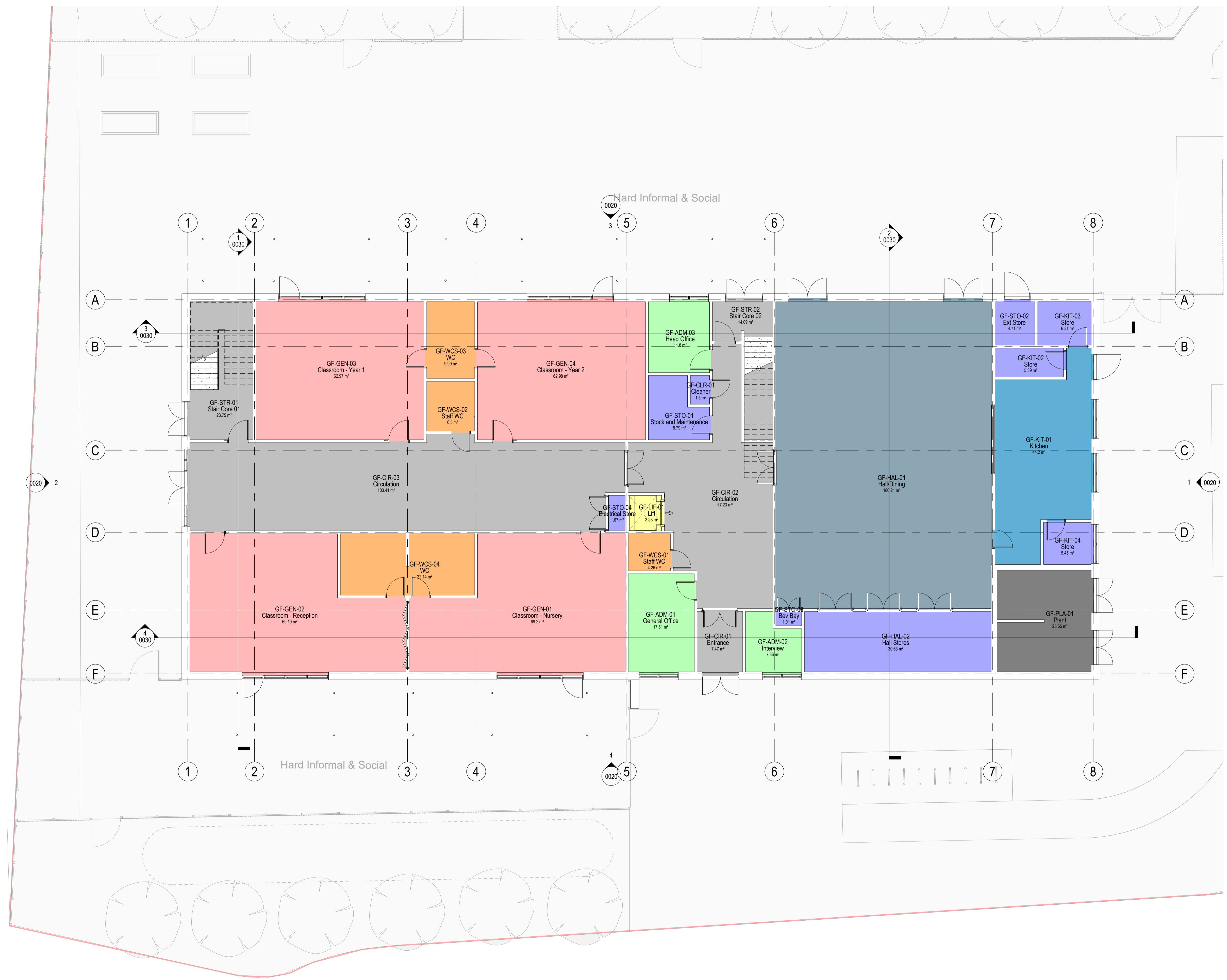
00 - Ground Floor Department Plan Scale: 1 : 100
