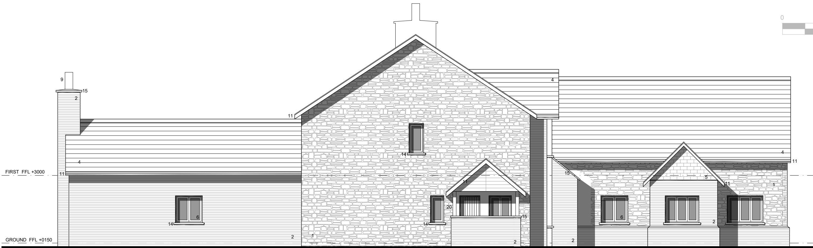
SIDE ELEVATION (NORTH FACING)
