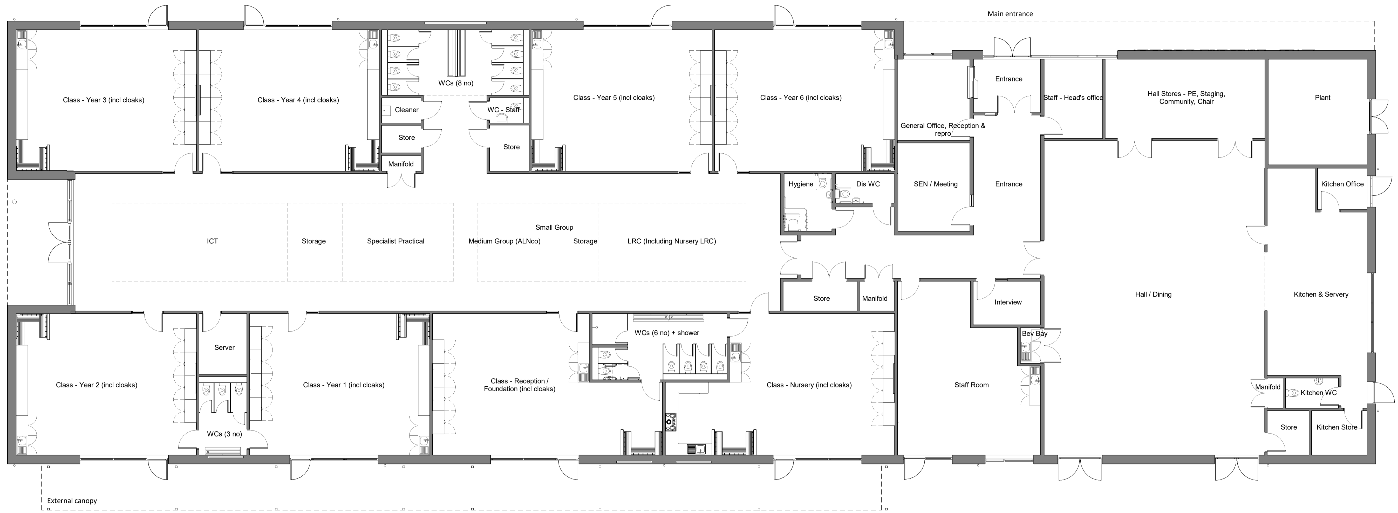
Proposed Floor Plan 1 : 100
