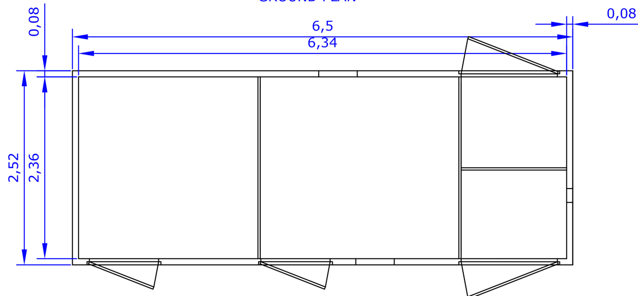
GROUND PLAN
