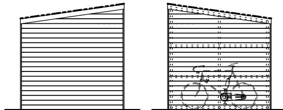
Side Elevation (C)
