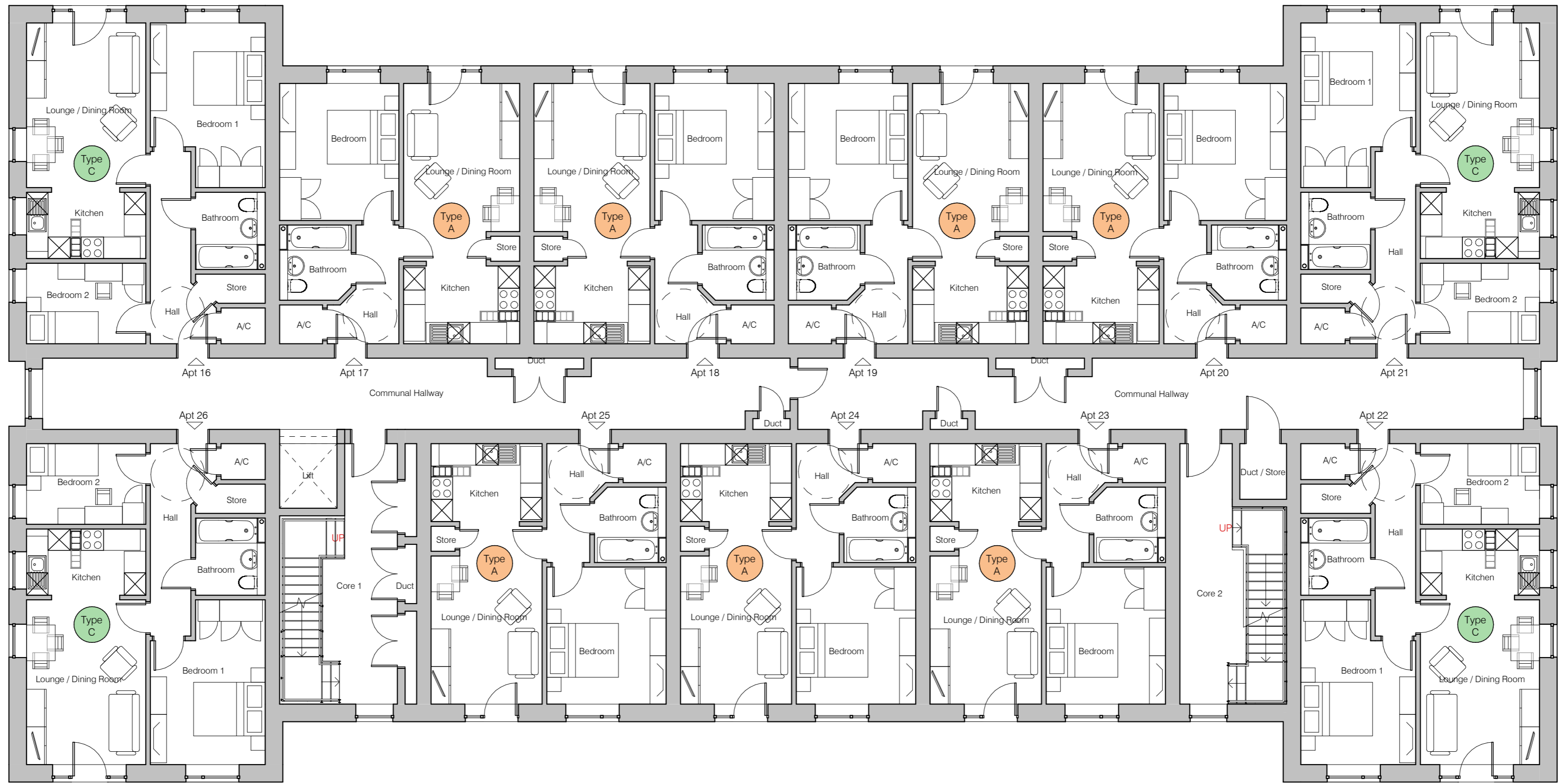
First Floor Plan 1 : 100
