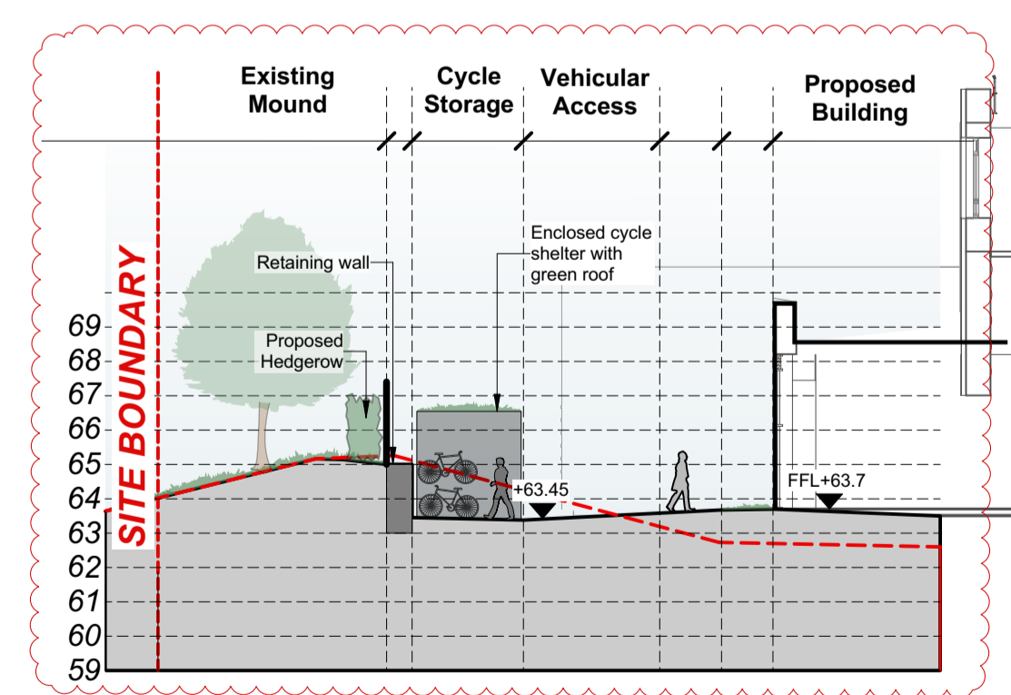
B-B Section - Through western boundary 00016 Scale: 200
