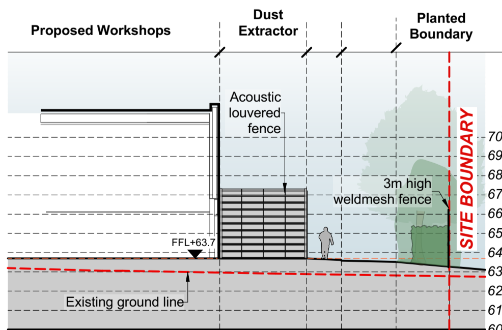
C-C Section - Through eastern boundary 00016 Scale: 200
