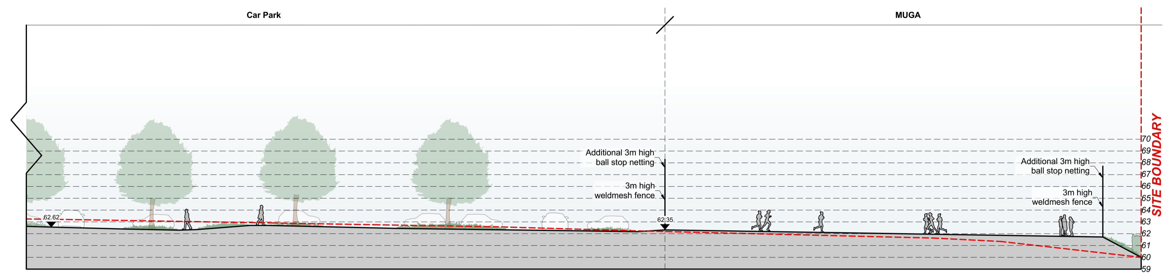
A-A Section - South to North 00016 Scale: 200
