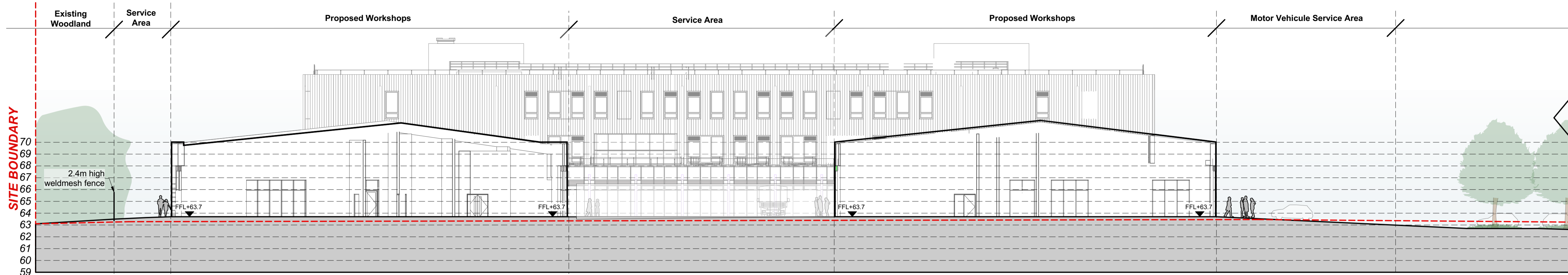
A-A Section - South to North 00016 Scale: 200
