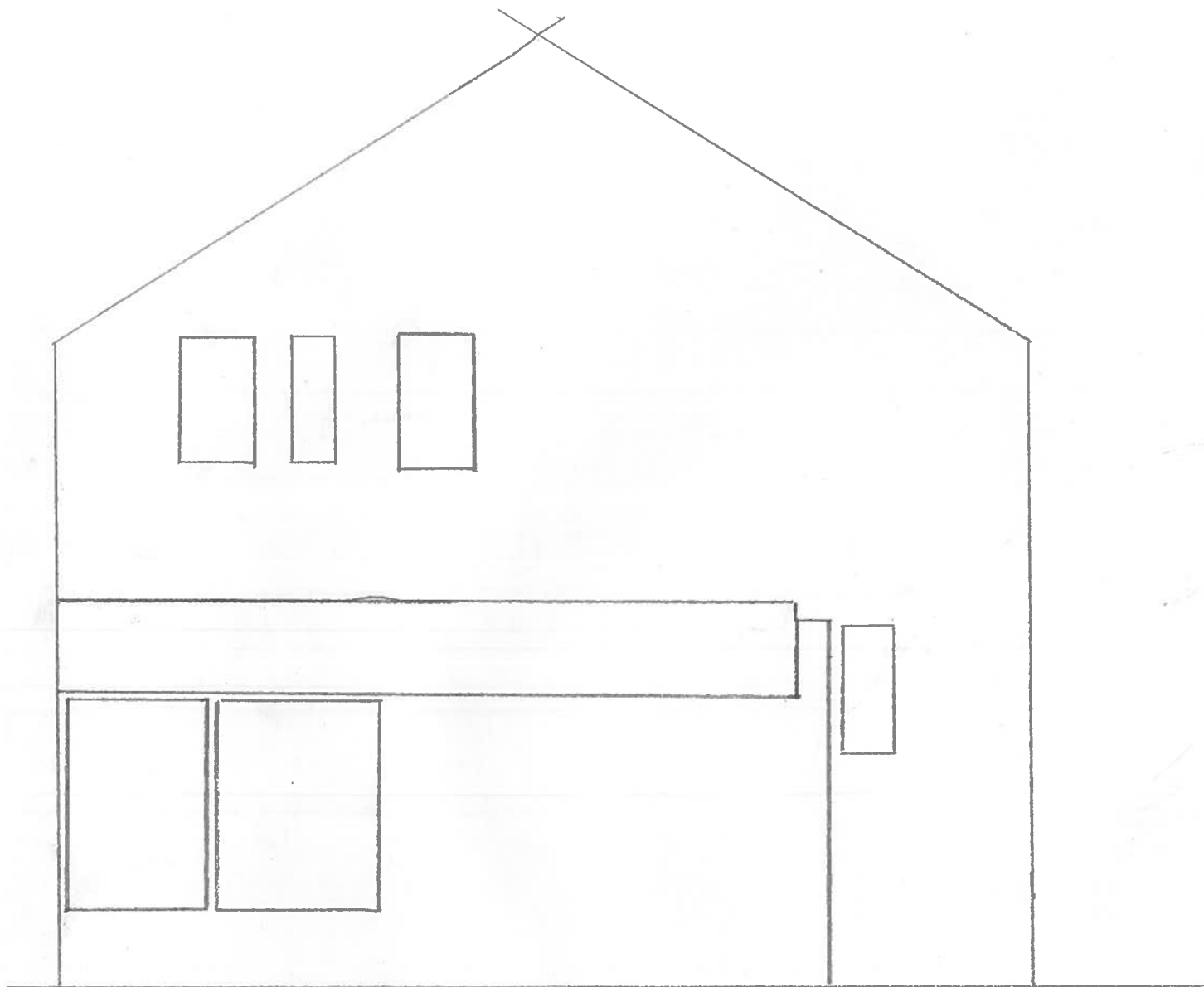
SIDE (EXISTING)
