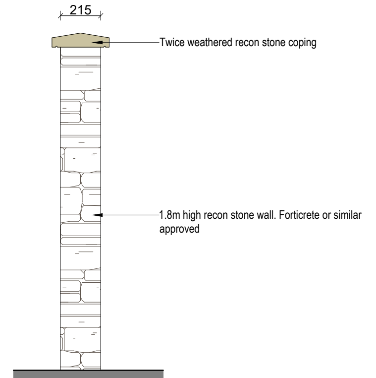
Section
