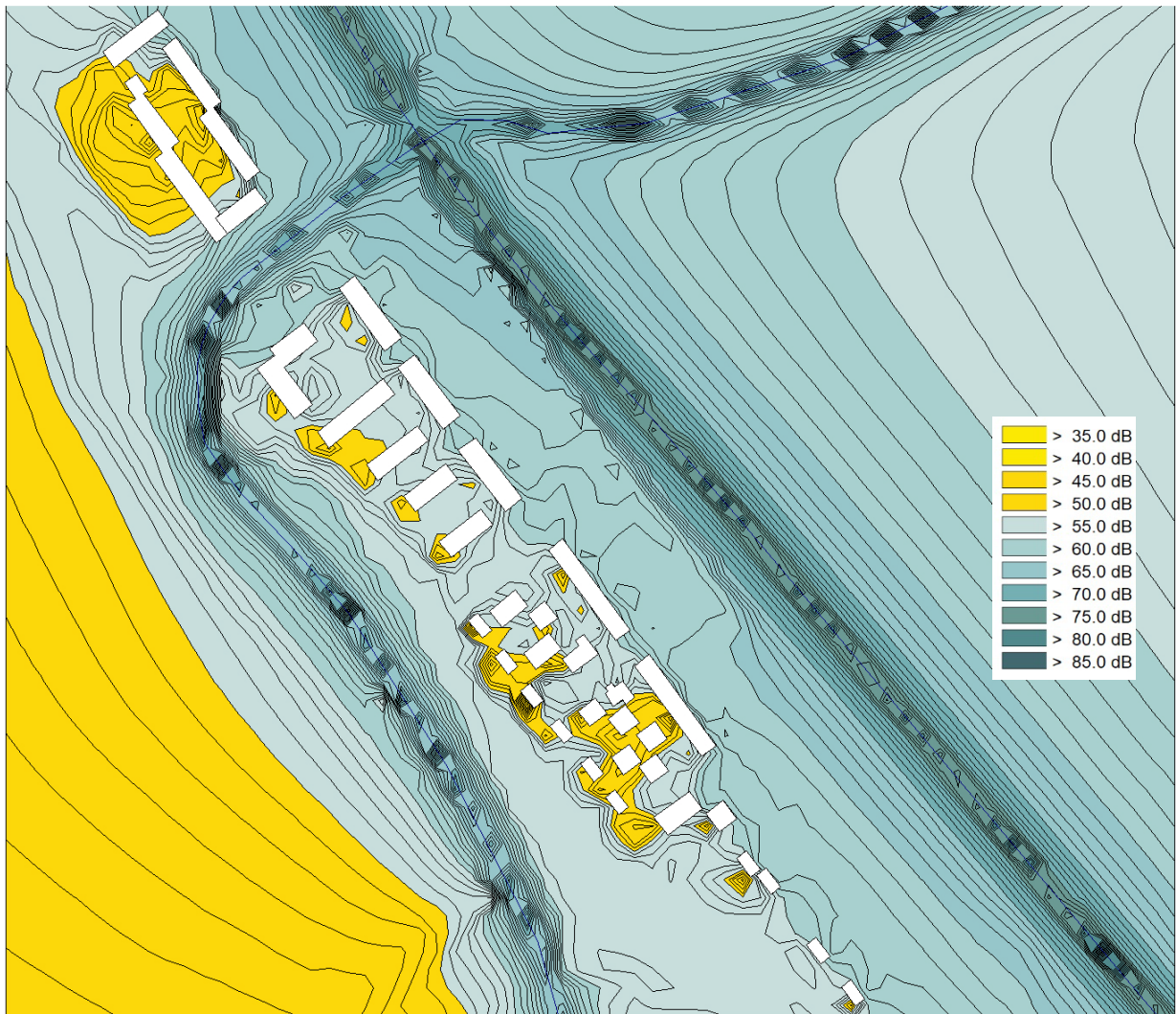
Figure 10.5: Noise map of development site – example layout option
