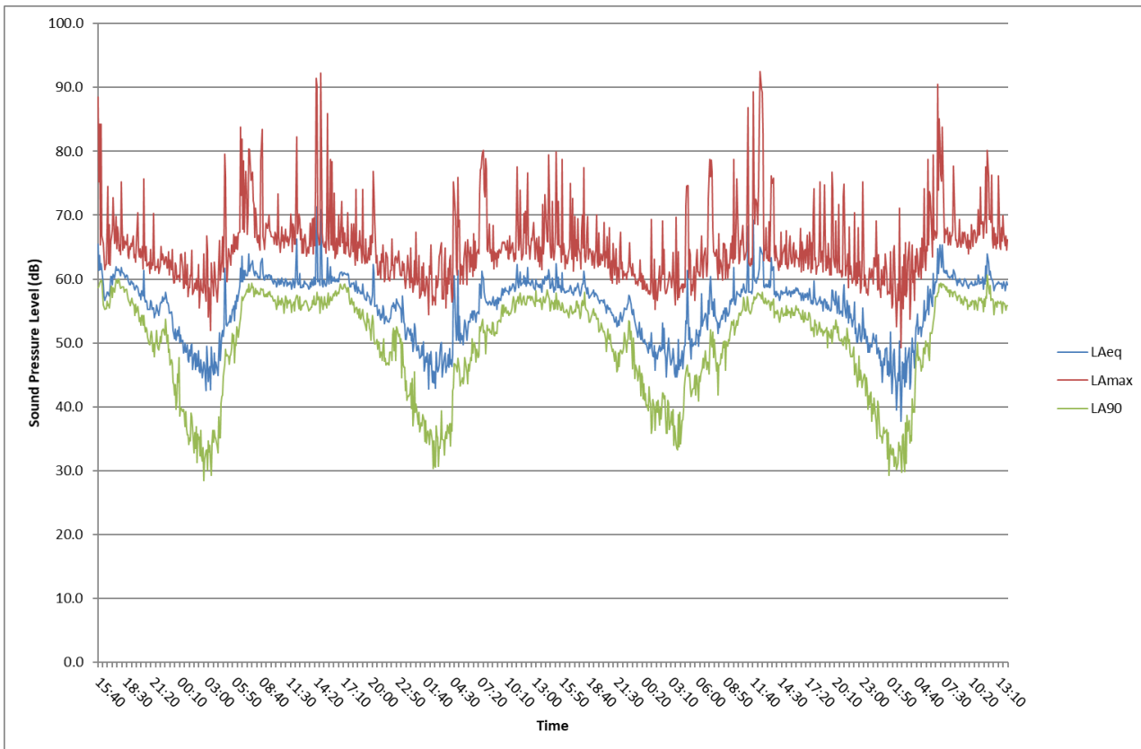
Figure 10.4: Graph of on-site environmental noise measurements (Fixed 2)
