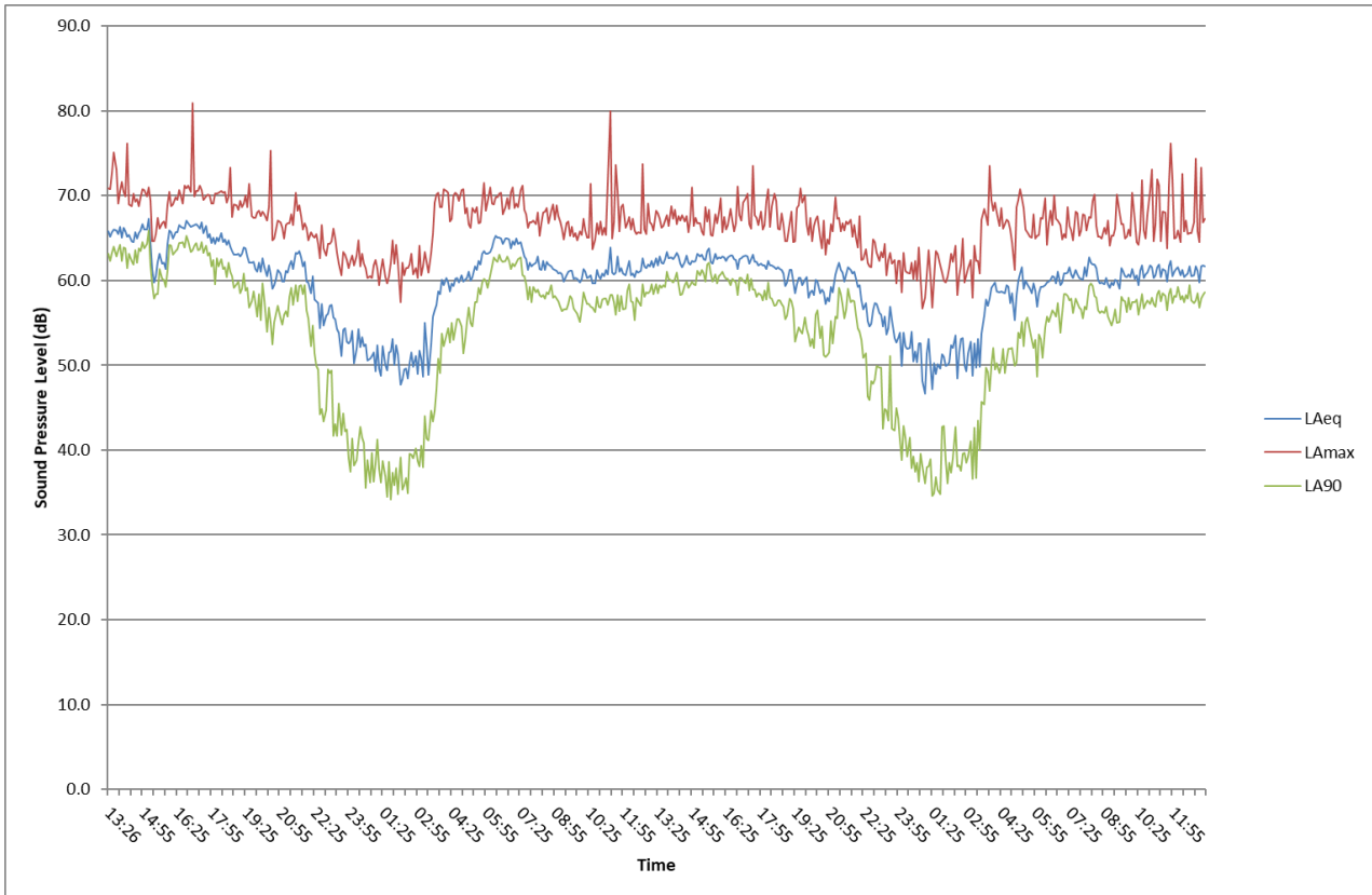
Figure 10.3: Graph of on-site environmental noise measurements (Fixed 1)
