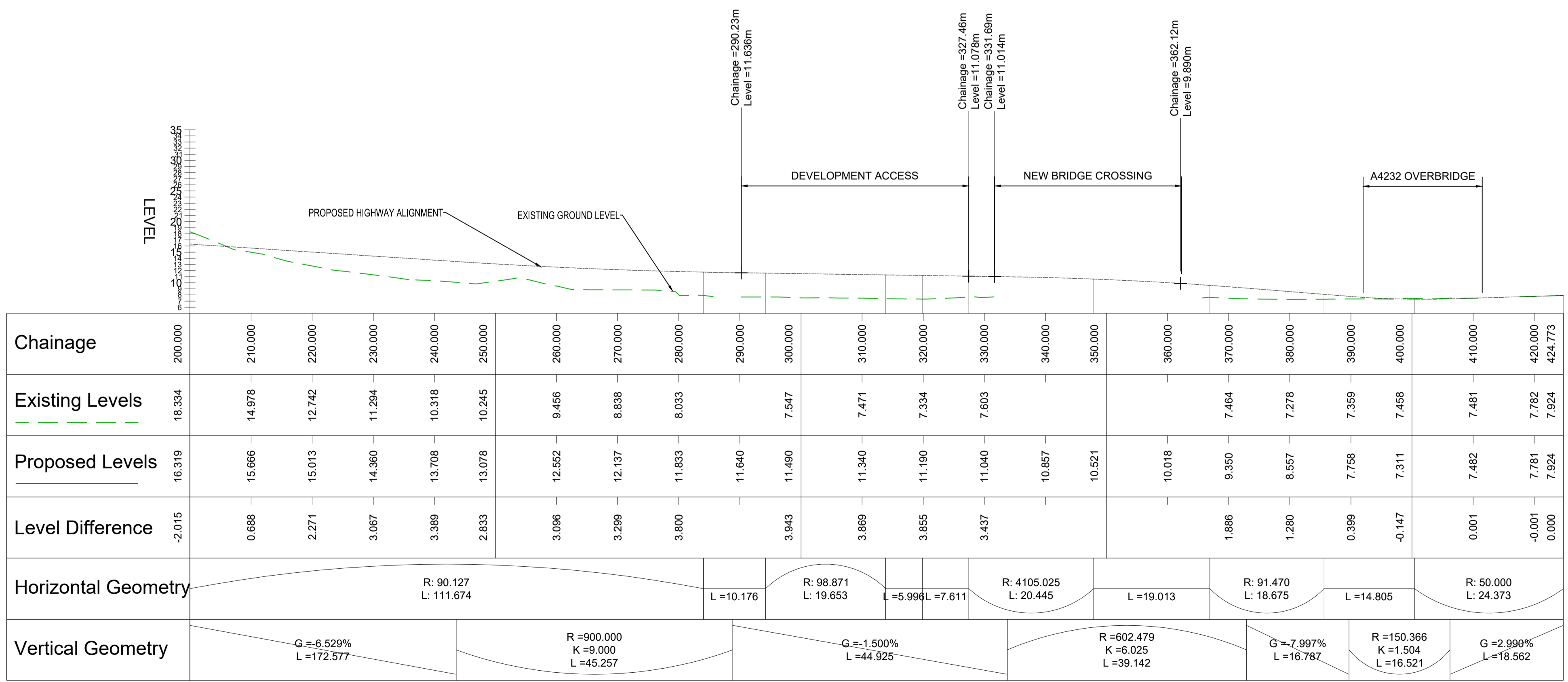
ROAD1 (CH.200-225) - LONGSECTION HORIZ 1:500, VERT 1:500. DATUM: 5.000m
