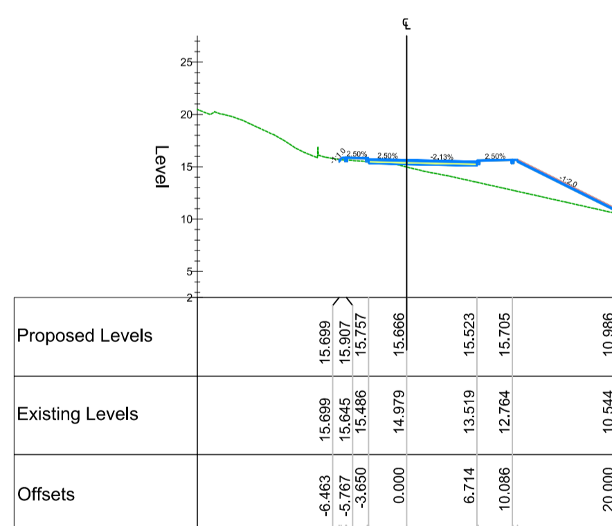
Chainage 210.000
