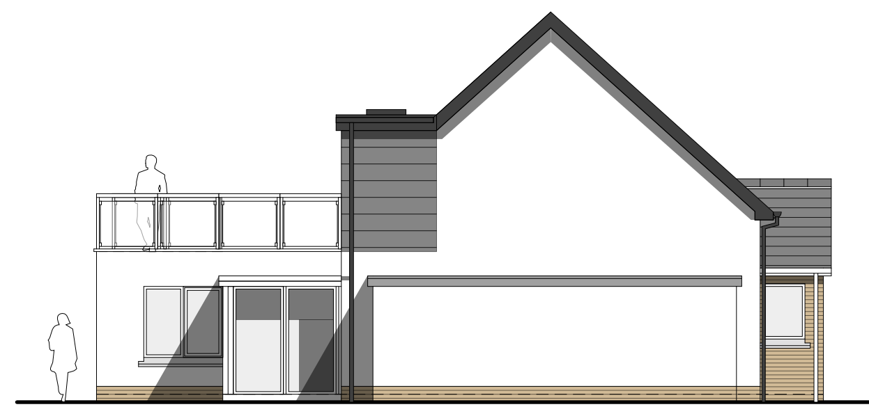
side 1 elevation (east facing)
