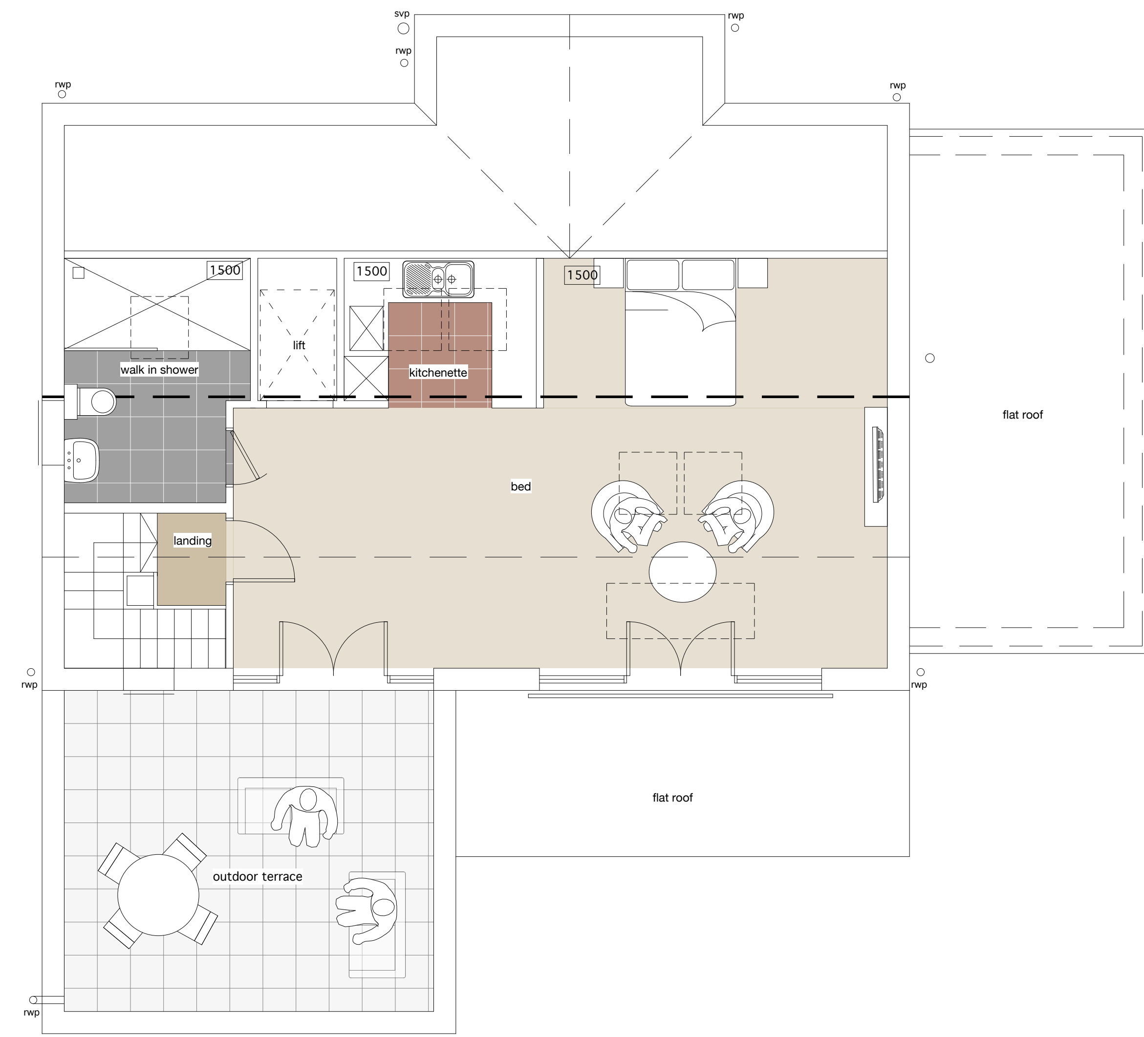
roof plan 1:50
