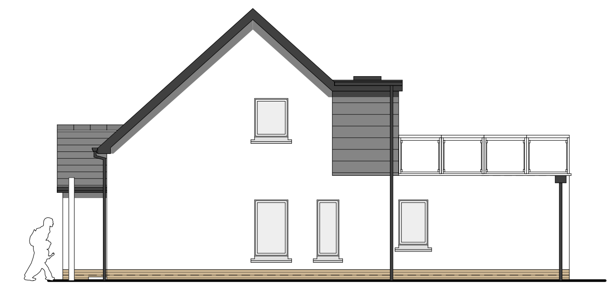
side 2 elevation (west facing)
