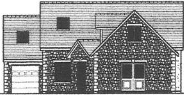
Front Elevation - Scale 1:100
