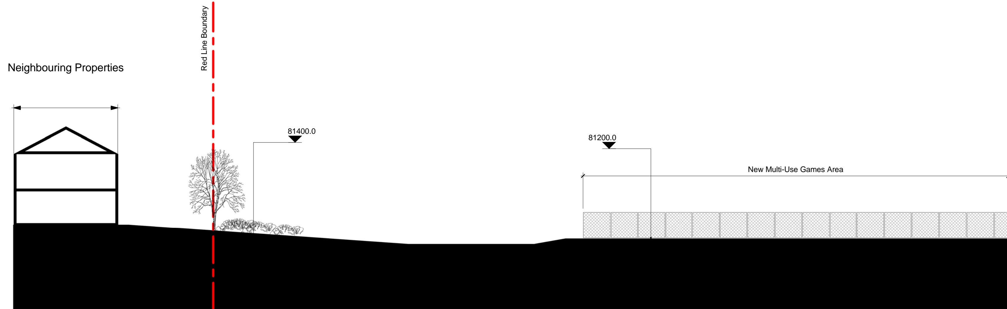
2 Section 1 Proposed 1:200
