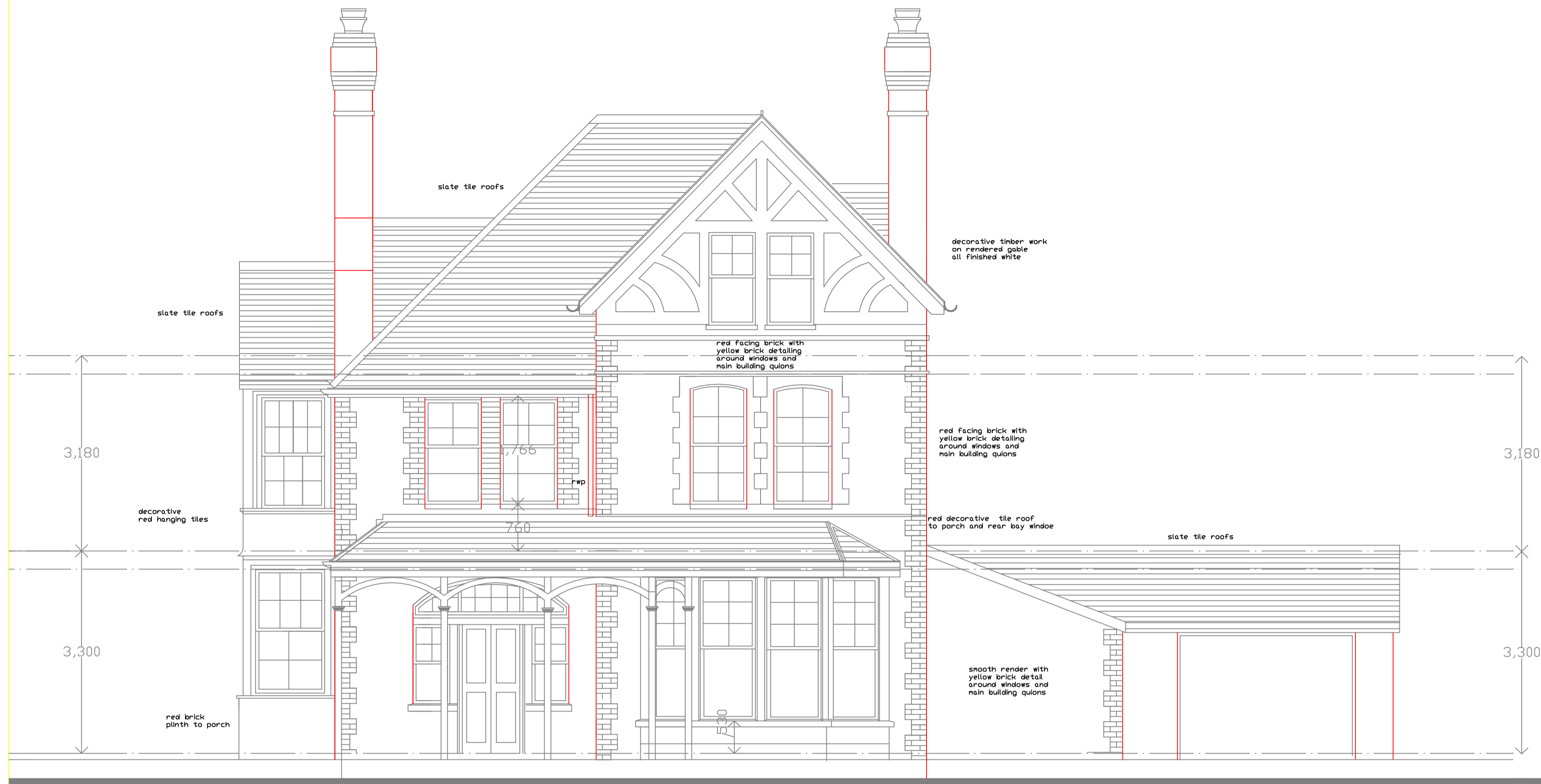
Existing Elevation to Garden
