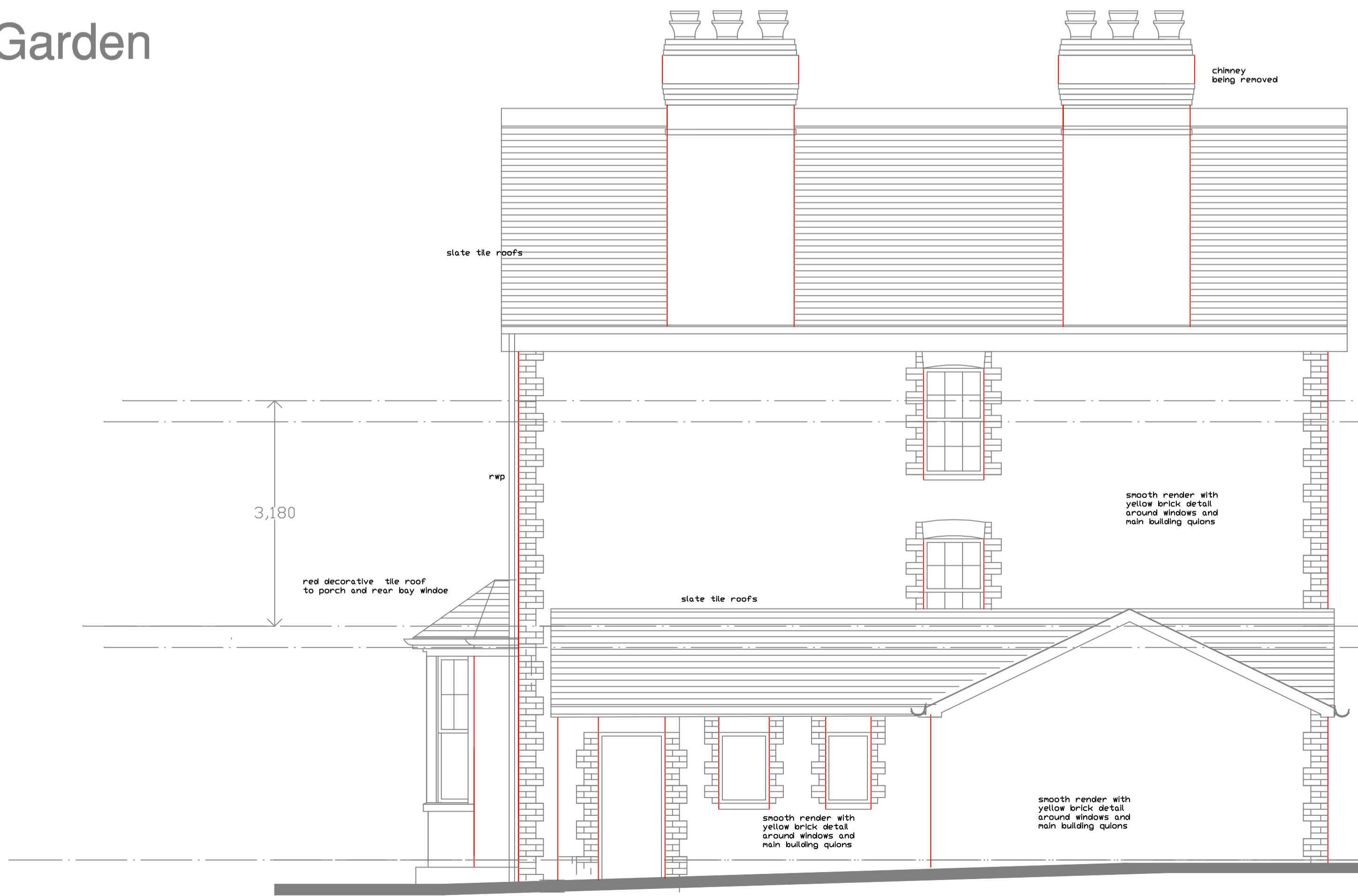
Existing Elevation to Road
