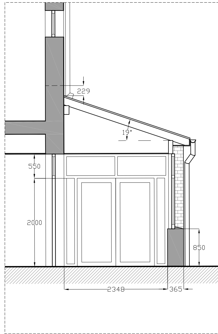
A/A section
