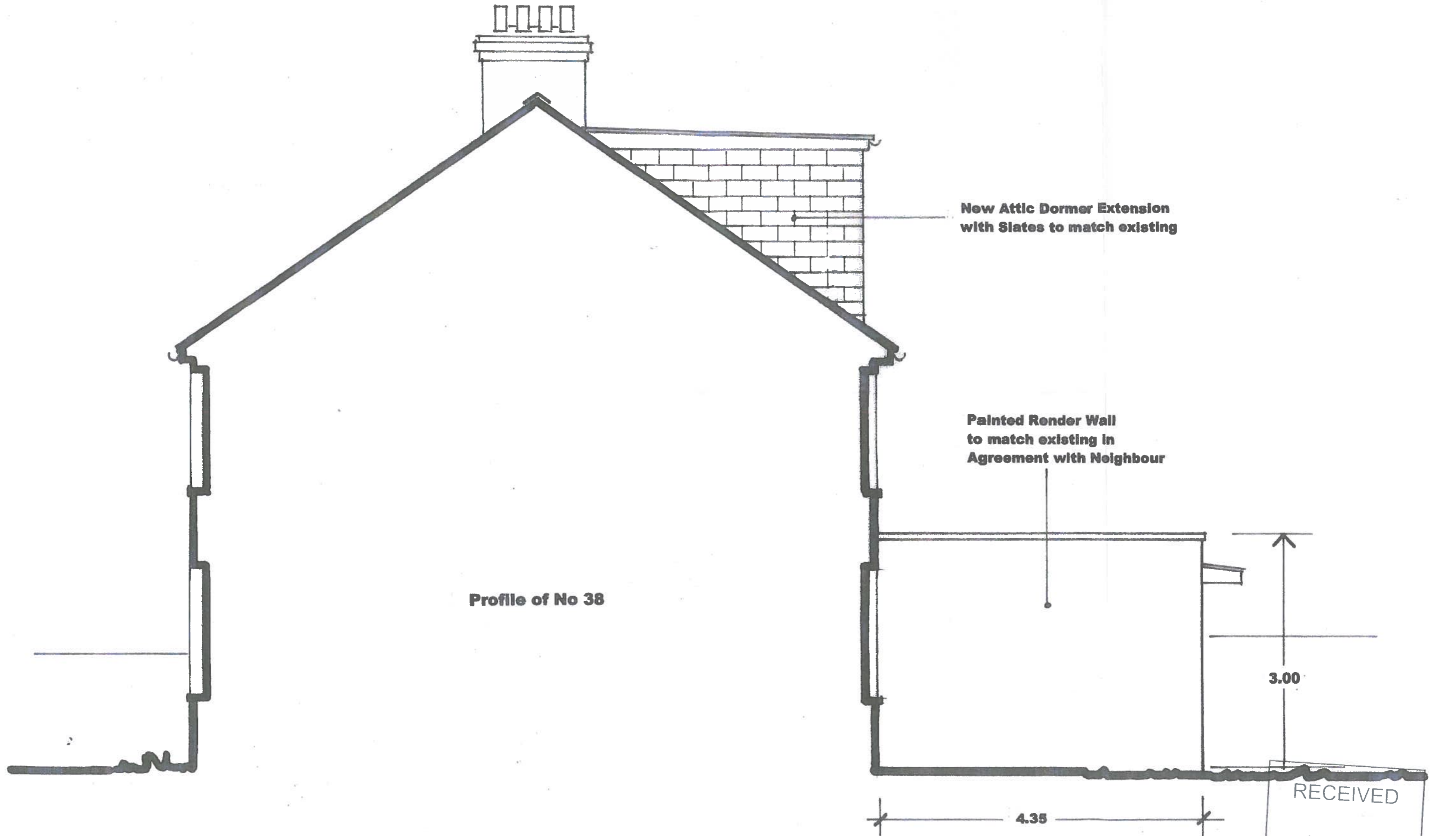
Proposed Side West Elevation Scale 1:50 @ A3
