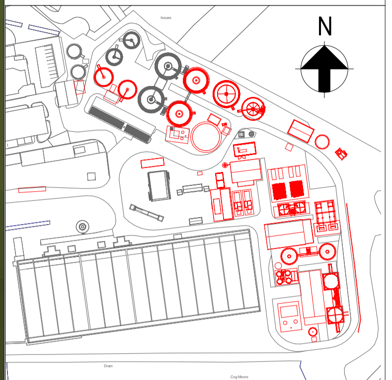
KEY PLAN 1:2500
