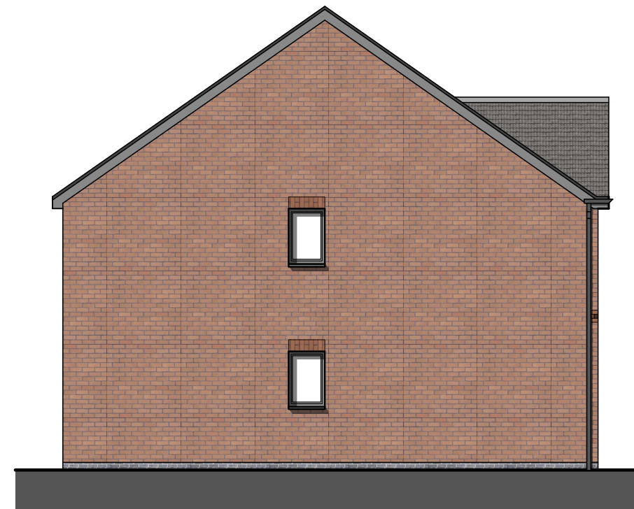
Hareford Plots: 2, 5, 11 (H), 13 (H) & 18 (H) Side Elevation
