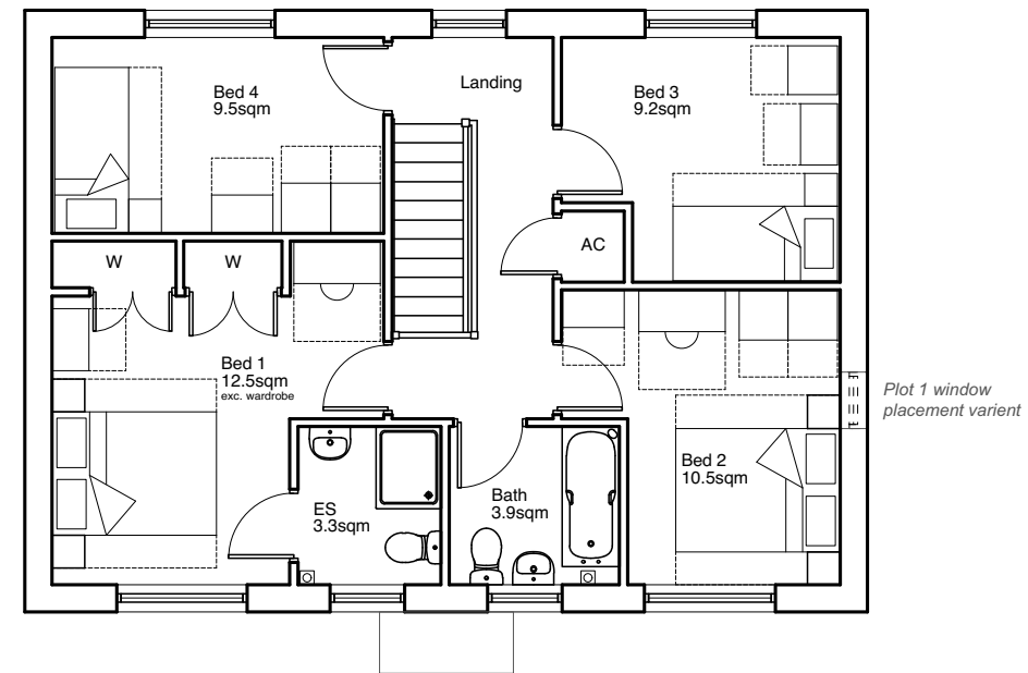
Lindford @ 127.2sqm Plots: 1, 9 (H), 14 (H), 19 (H), 25 & 40 First Floor
