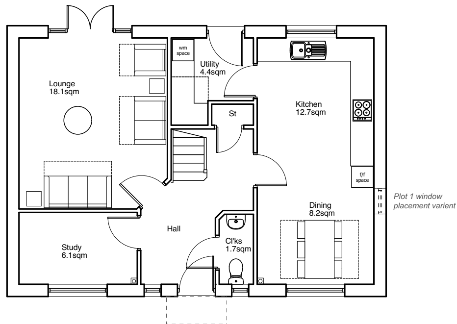
Lindford @ 127.2sqm Plots: 1, 9 (H), 14 (H), 19 (H), 25 & 40 Ground Floor
