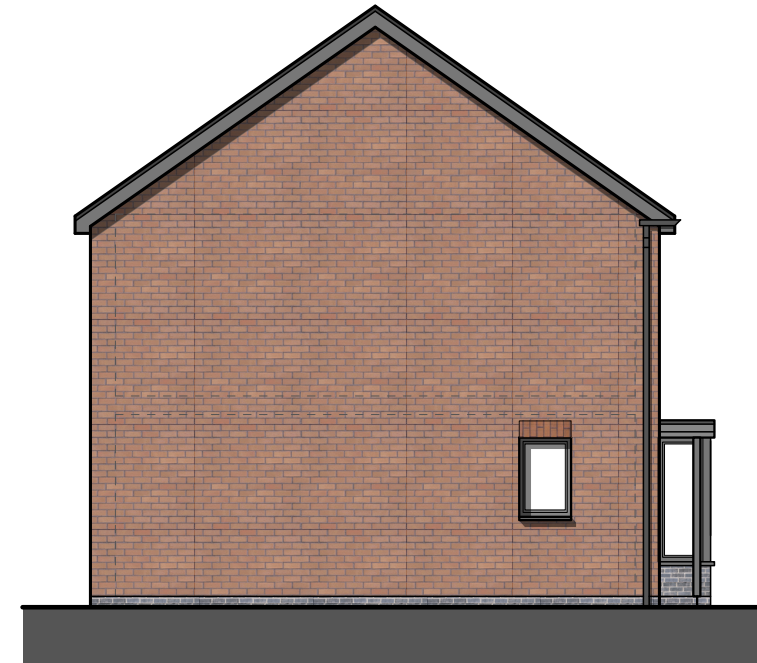
Hatton End Plot: 29 Side Elevation
