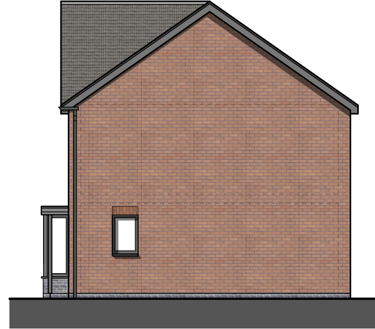
Hatton End Plot: 28 Side Elevation
