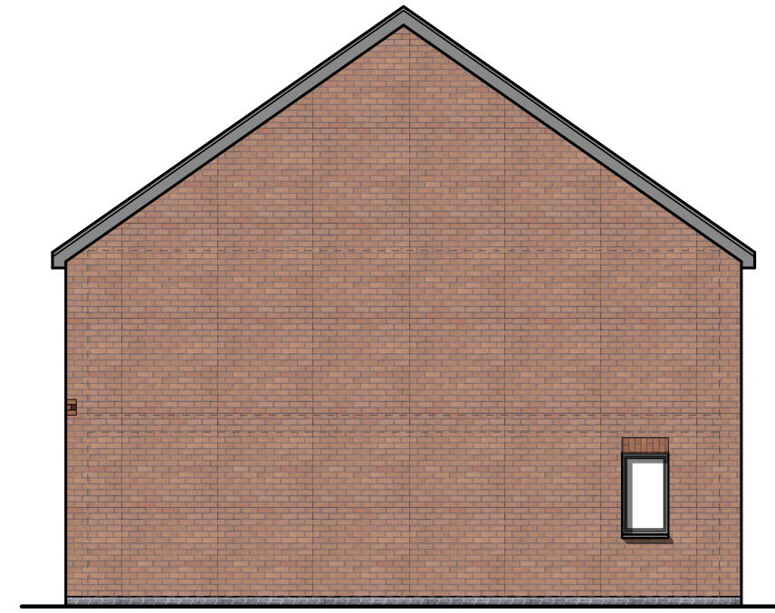
2Bed LCHO End Plots: 38 & 54 Side Elevation
