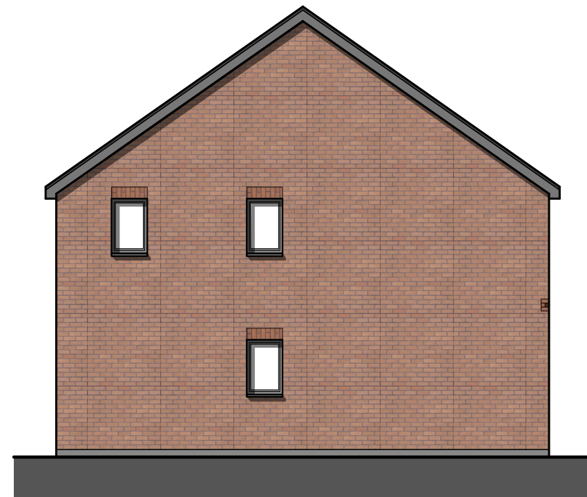
Holmewood Plots: 32 (H), 33, 42 (H) & 43 Side Elevation
