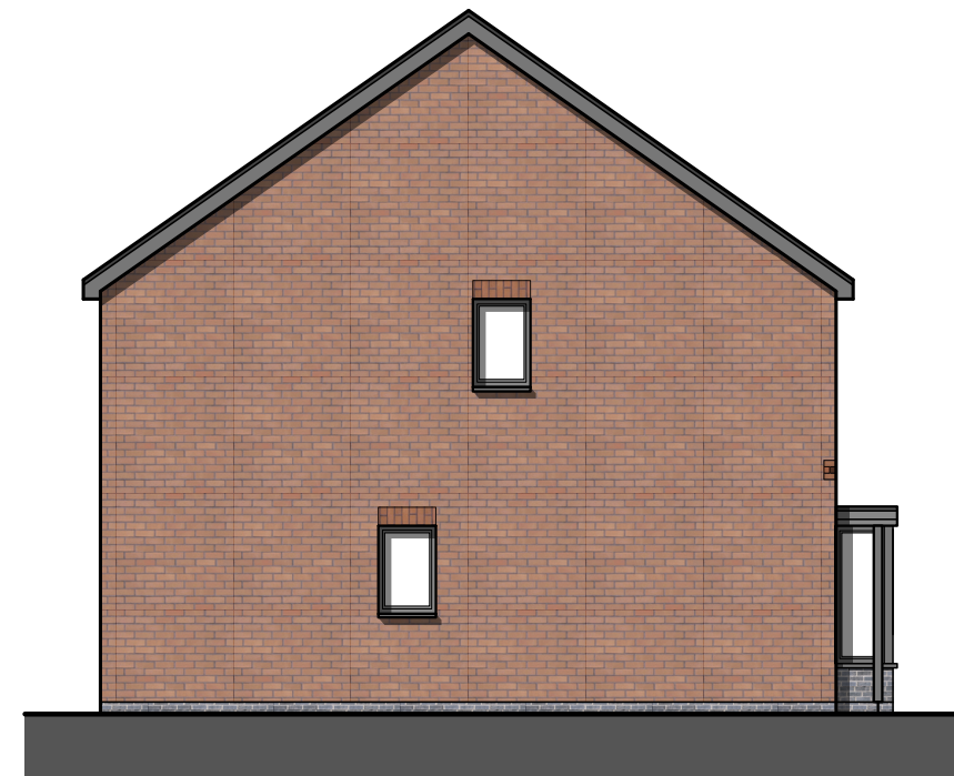
Pemberton Plots: 35 & 44 (H) Side Elevation
