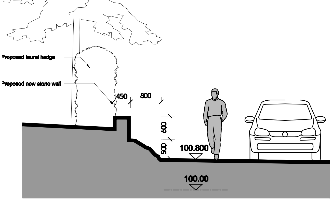
SECTION B - 1:50
