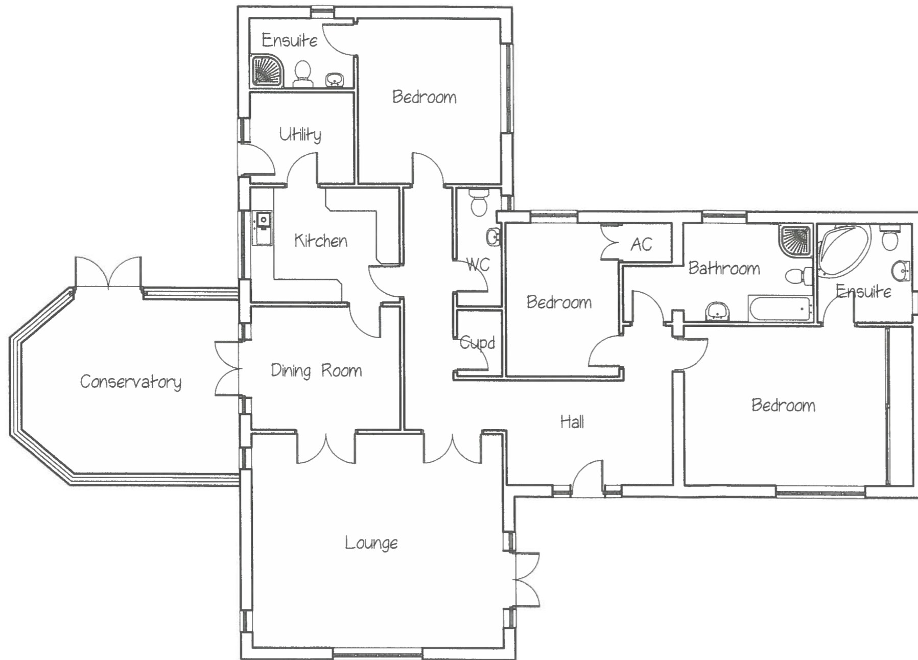
Existing floor plan Scale 1:100
