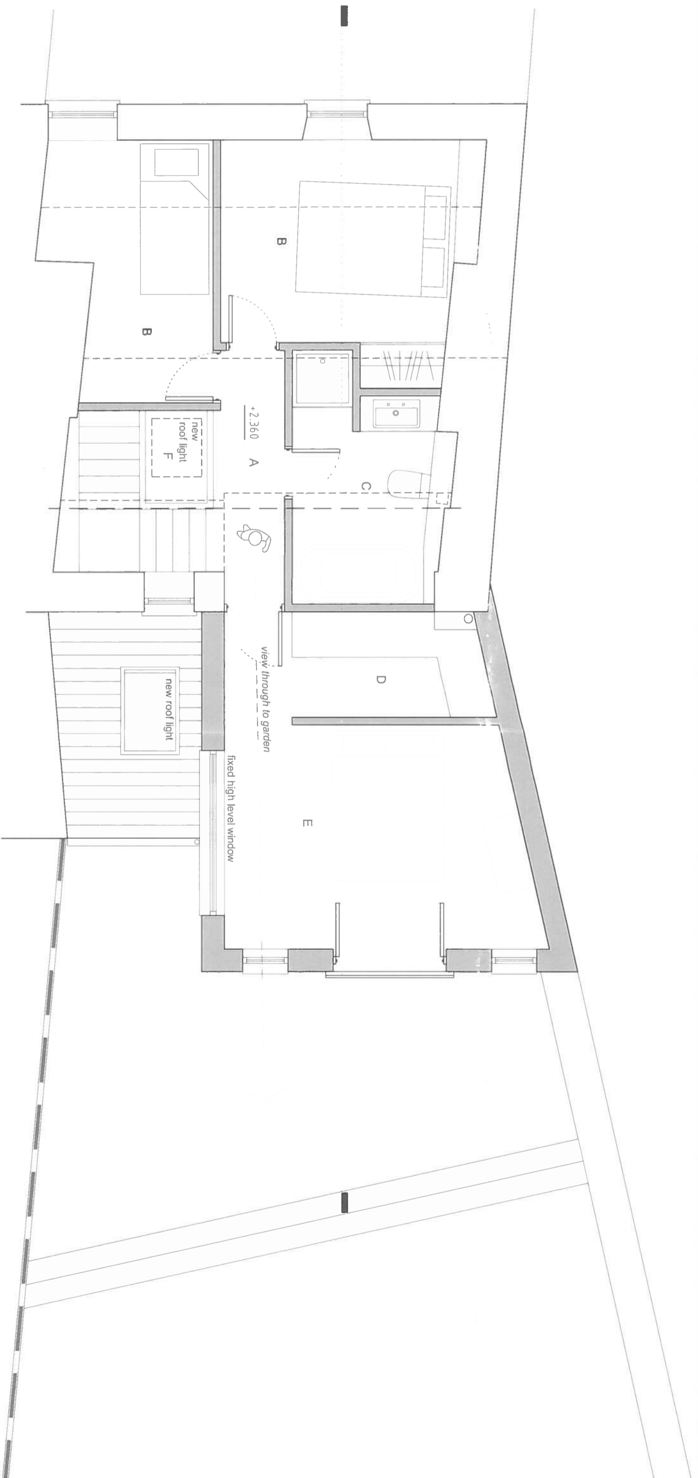
PROPOSED FIRST FLOOR PLAN 1:50
