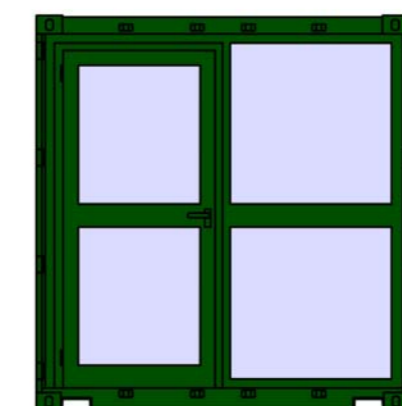
Reception Building Elevation 4 (Open) (1:50)
