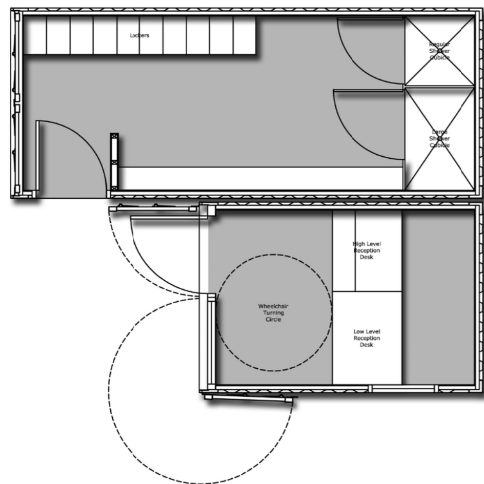
Changing Building and Reception Building Plans Grouped Together (1:50)
