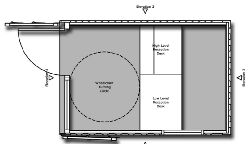
Reception Building Plan (1:50)
