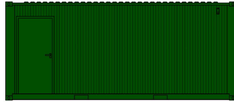
Changing Building Elevation 1 (1:50)
