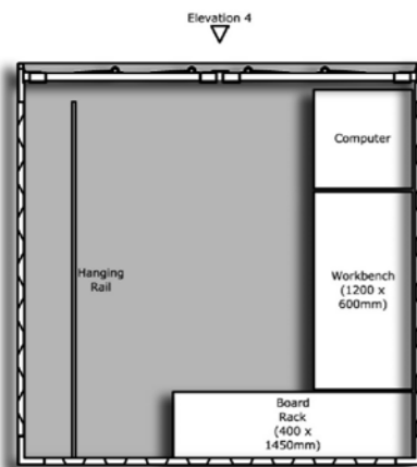
Equipment Store Plan
