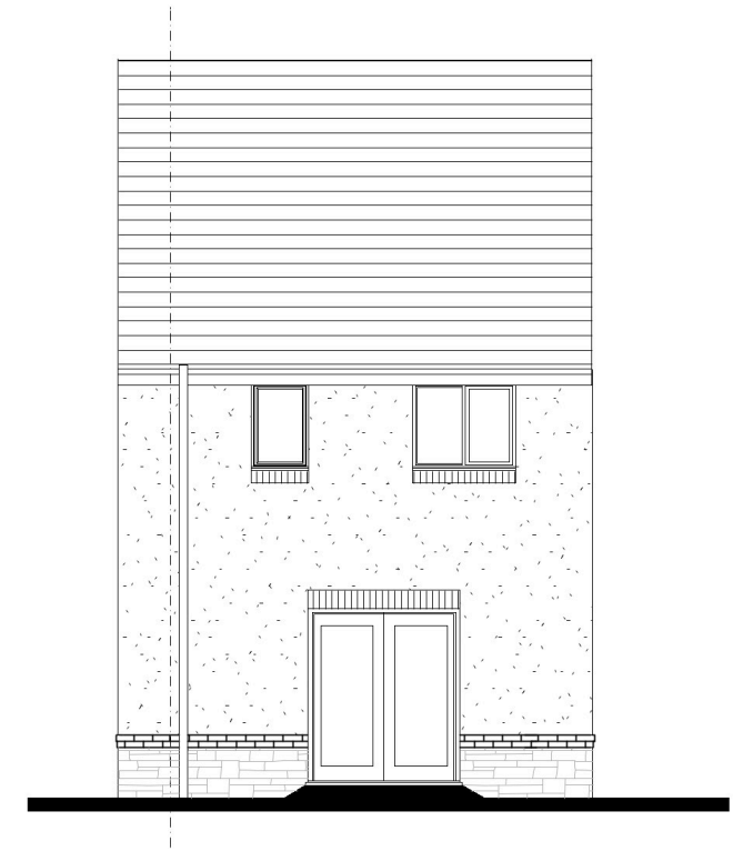
REAR ELEVATION
