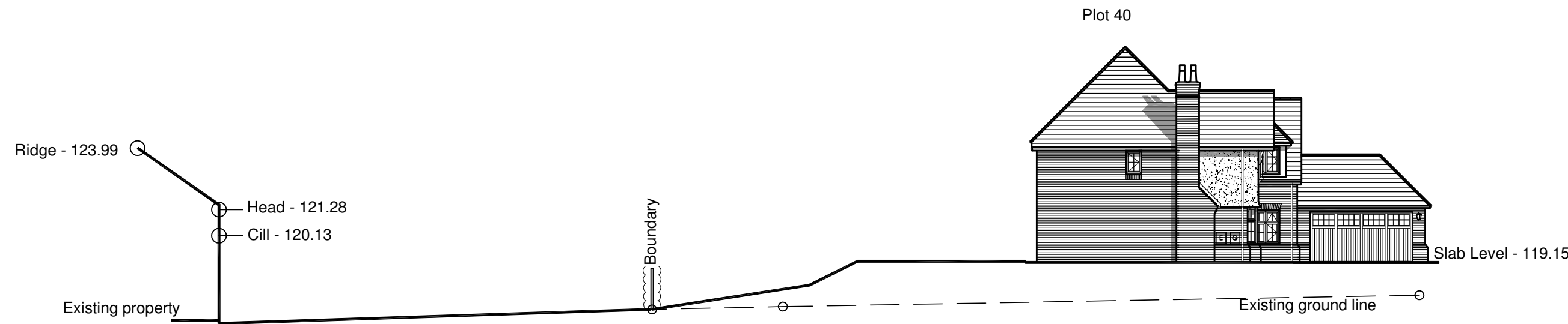
Site Section 1
