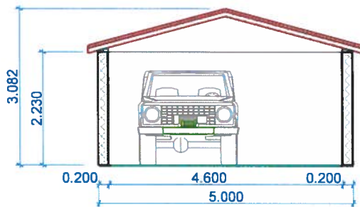
S-01 Building Section 1:100
