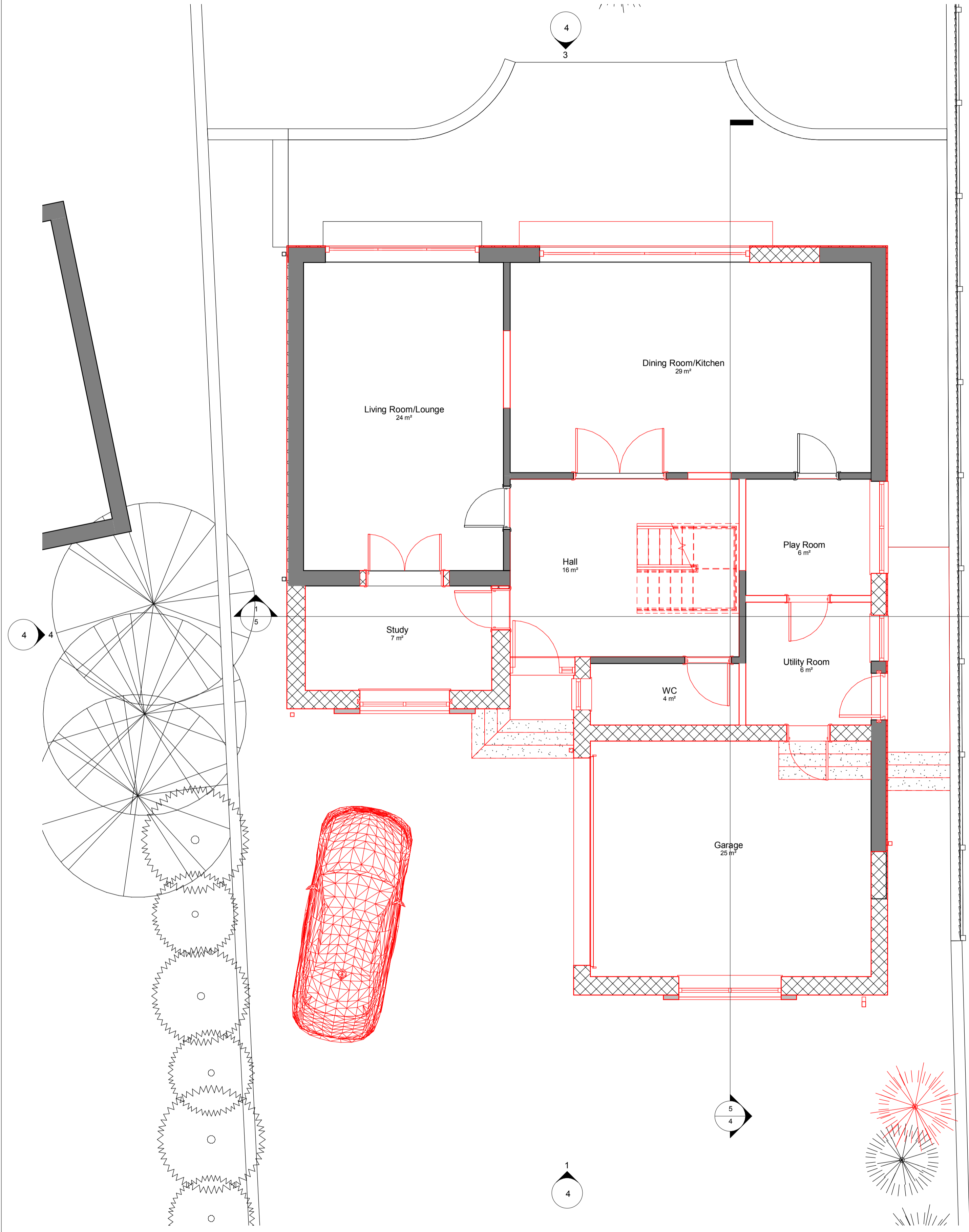
00-Ground Floor-proposed 1 : 50
