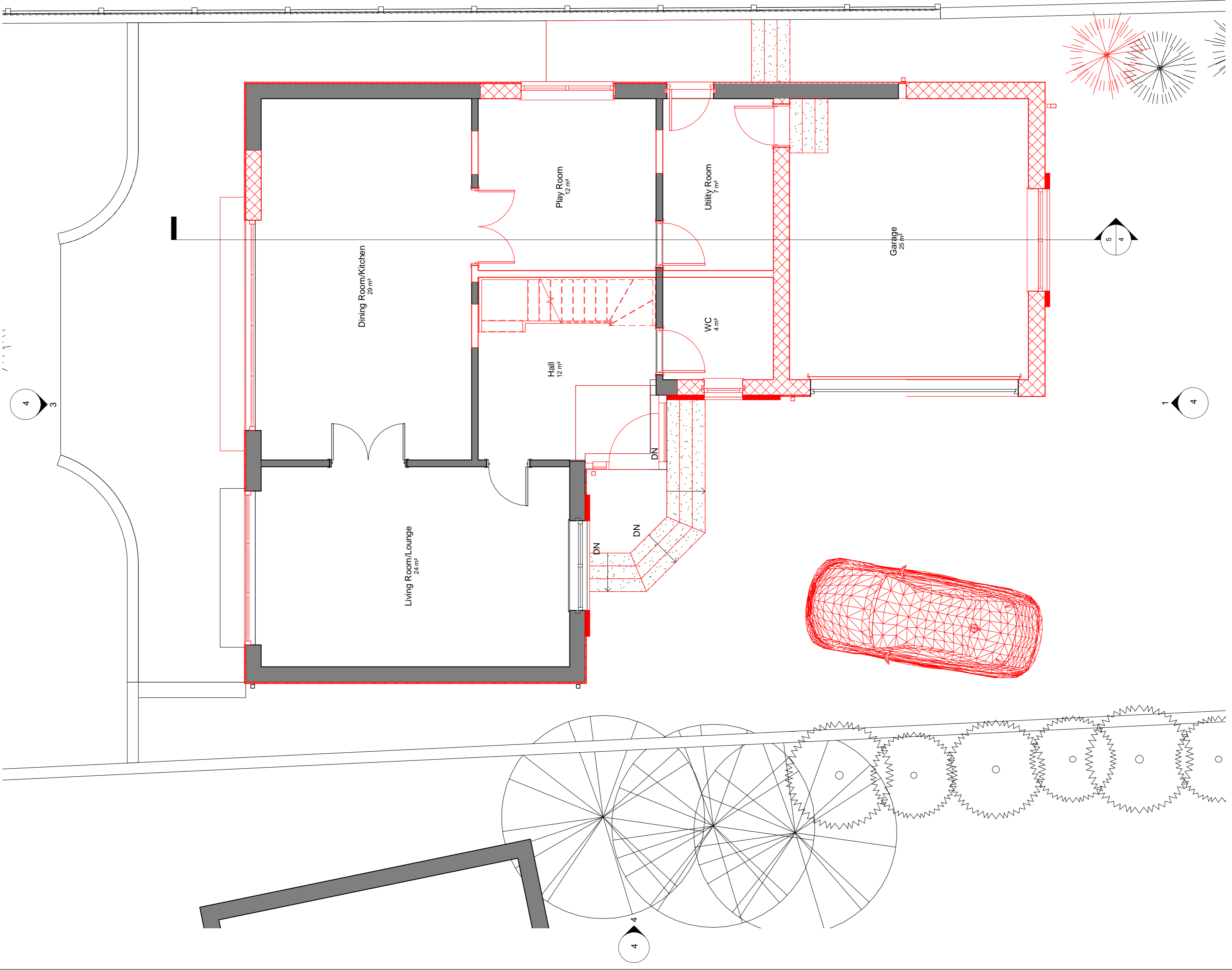
00-Ground Floor-proposed 1 : 50
