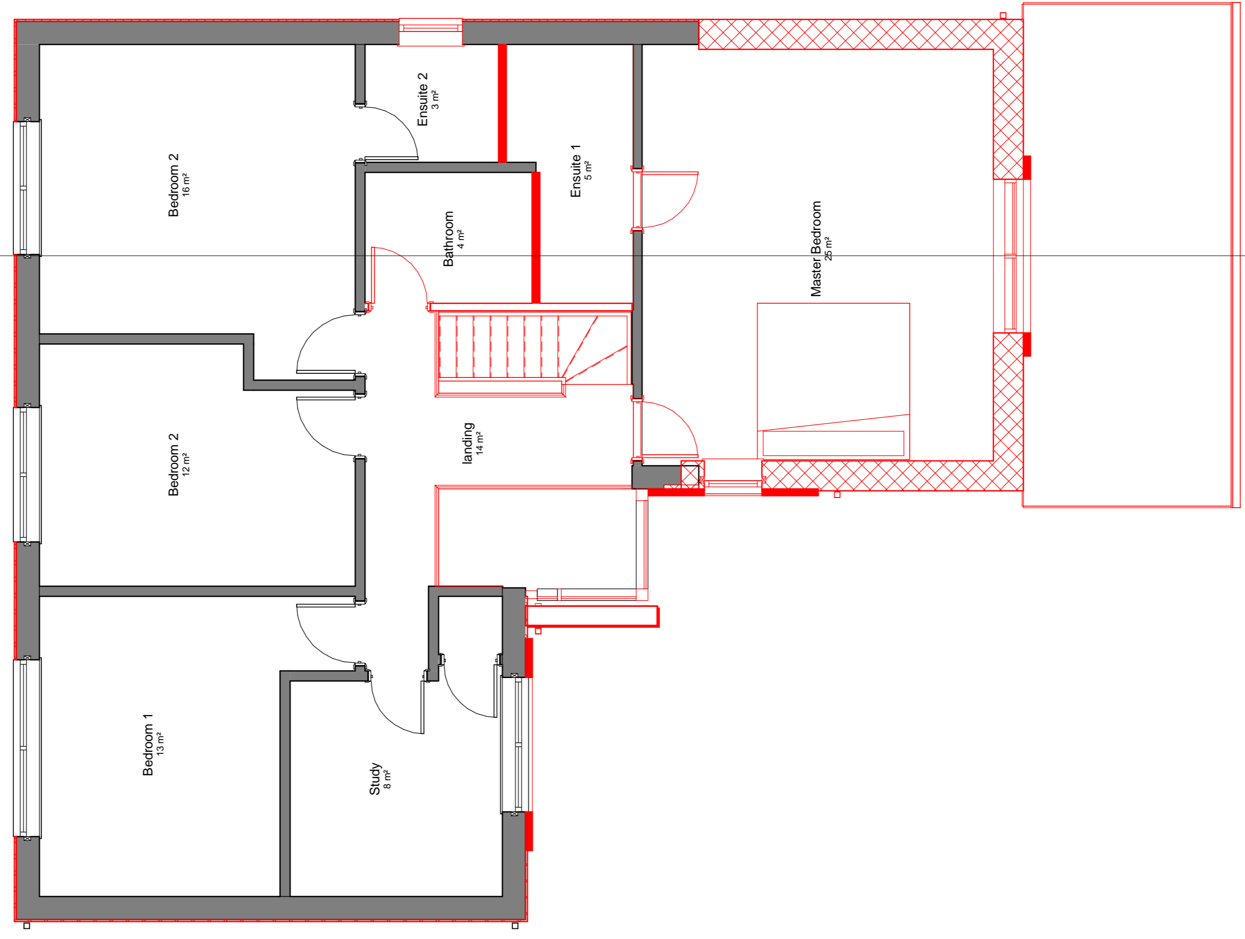
01-first floor-proposed 1 : 50
