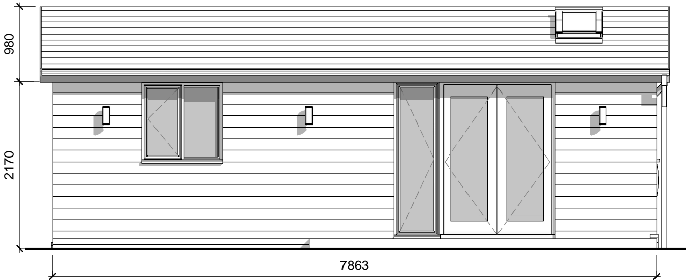
2 Front Elevation 1 : 50
