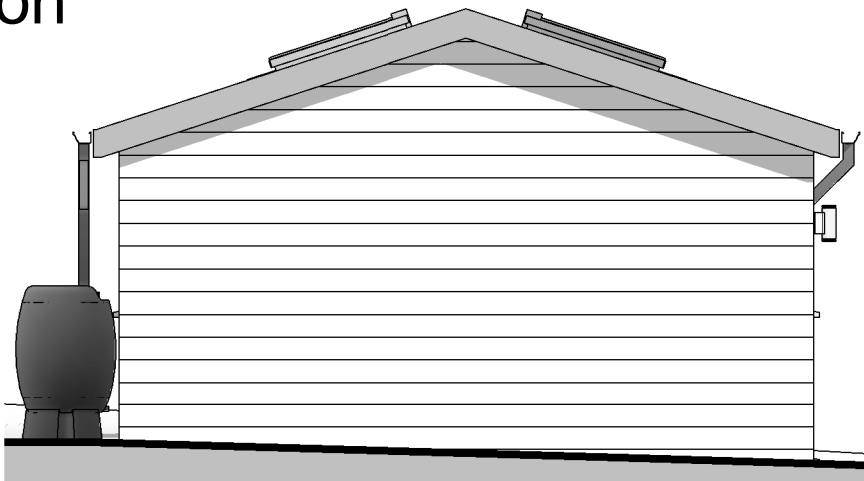
1 East Elevation 1 : 50
