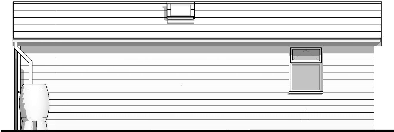
3 Rear Elevation 1 : 50
