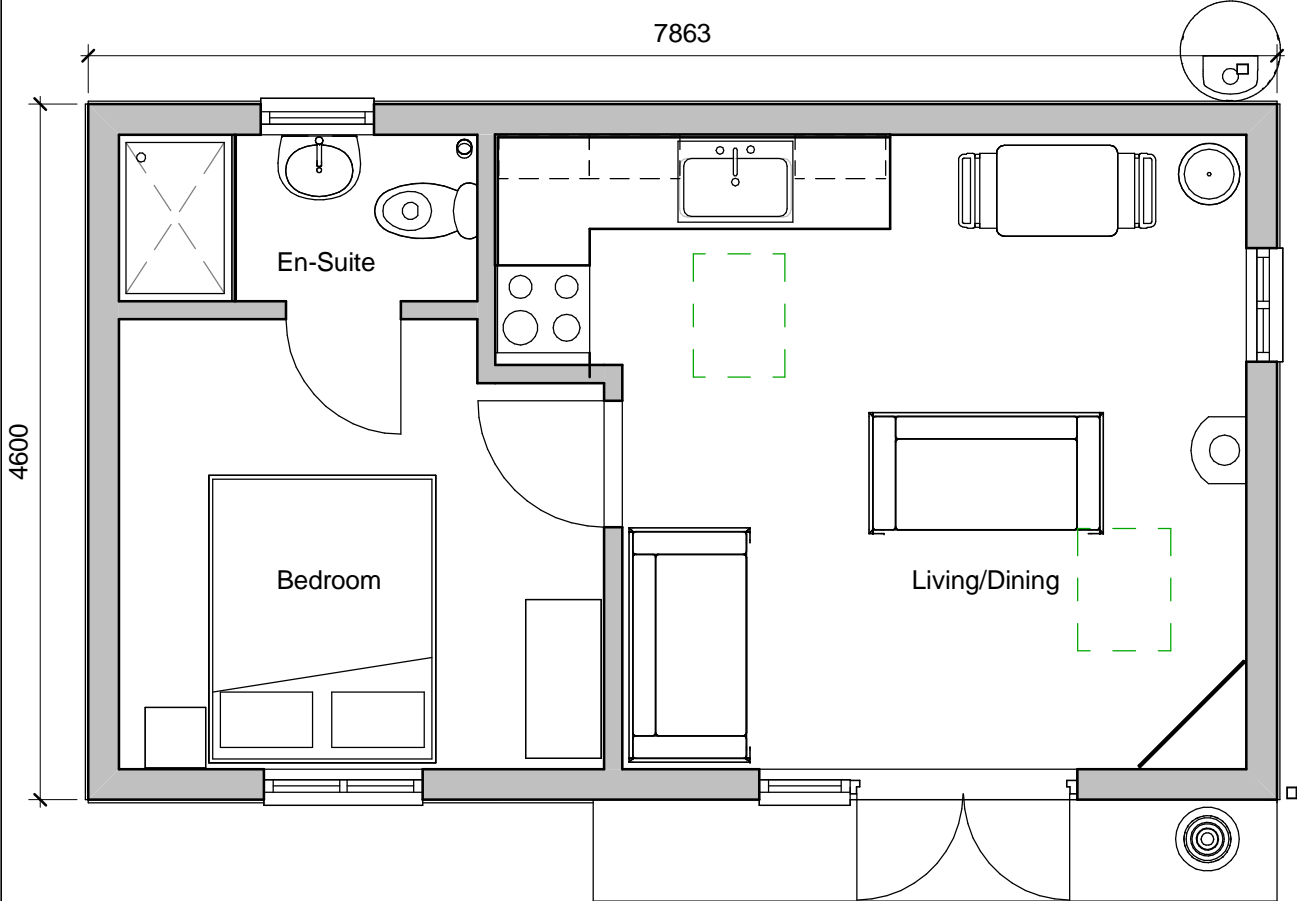
5 01 Proposed Floor Plan 1 : 50
