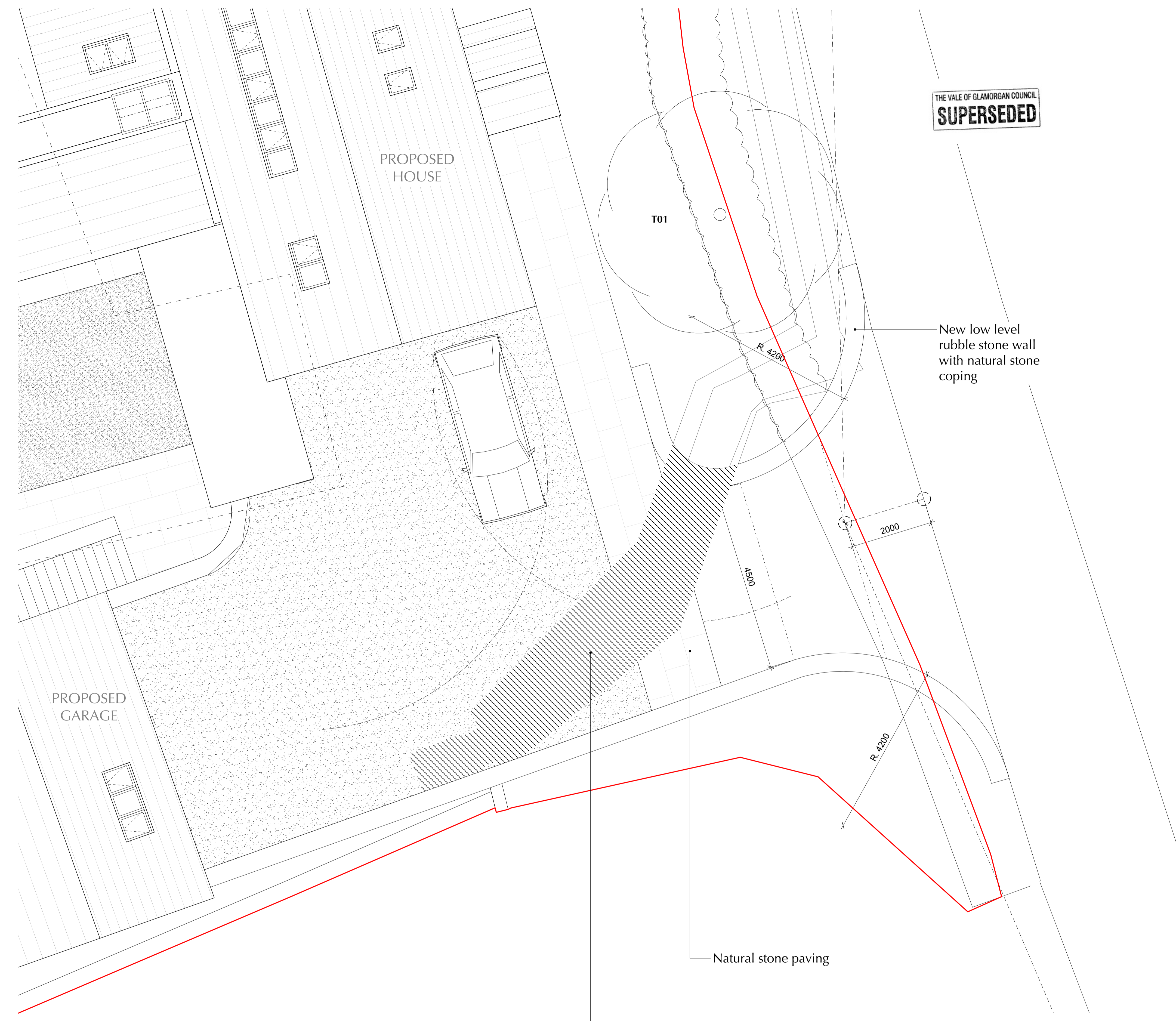
SITE ACCESS PLAN SCALE 1:50 @ A1, 1:100 @ A3
