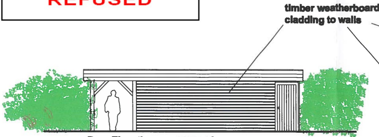
Rear Elevation as proposed
