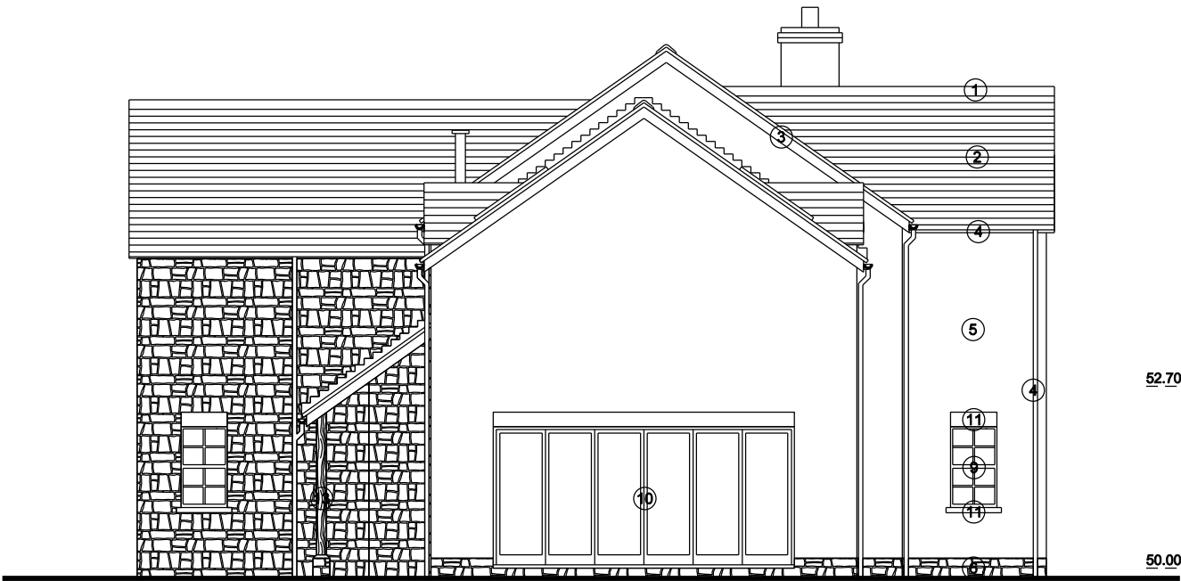
Proposed Side (West) Elevation
