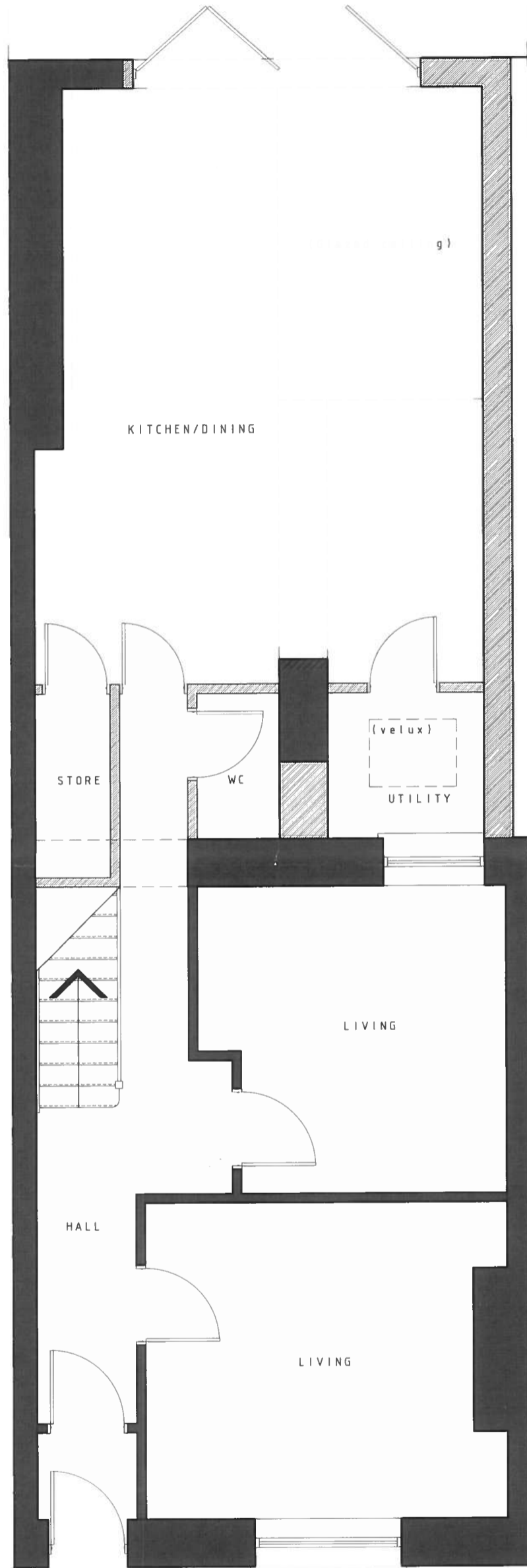
As built ground floor plan 1:50
