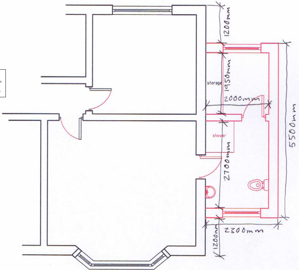
PART PLAN
