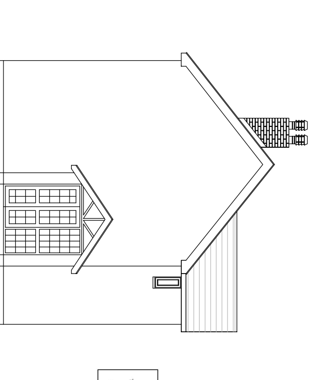
Left hand elevation as existing
