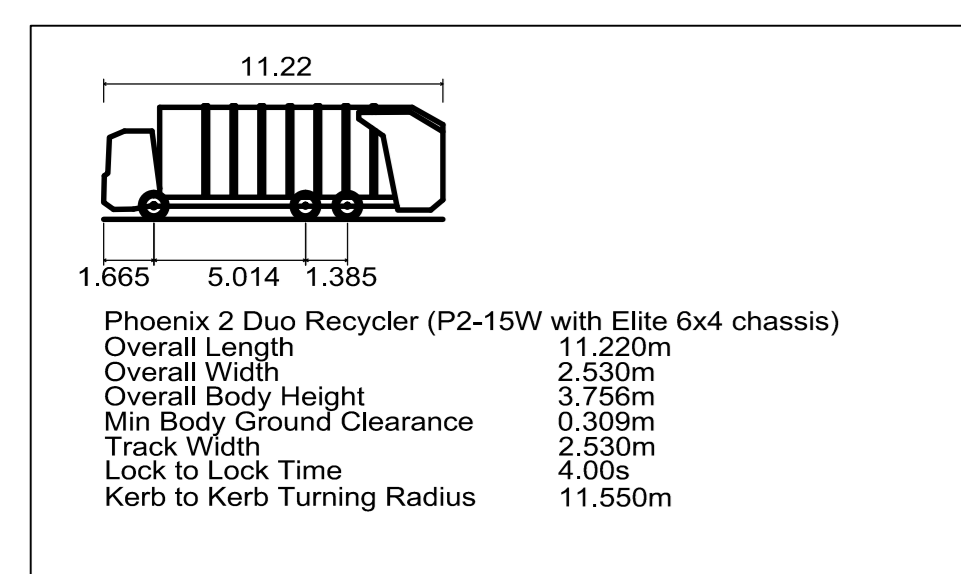
Design Vehicle 11.2m Refuse
