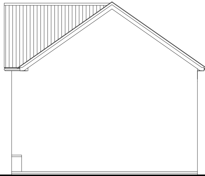
SIDE ELEVATION
