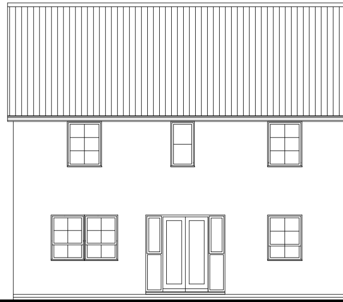
REAR ELEVATION
