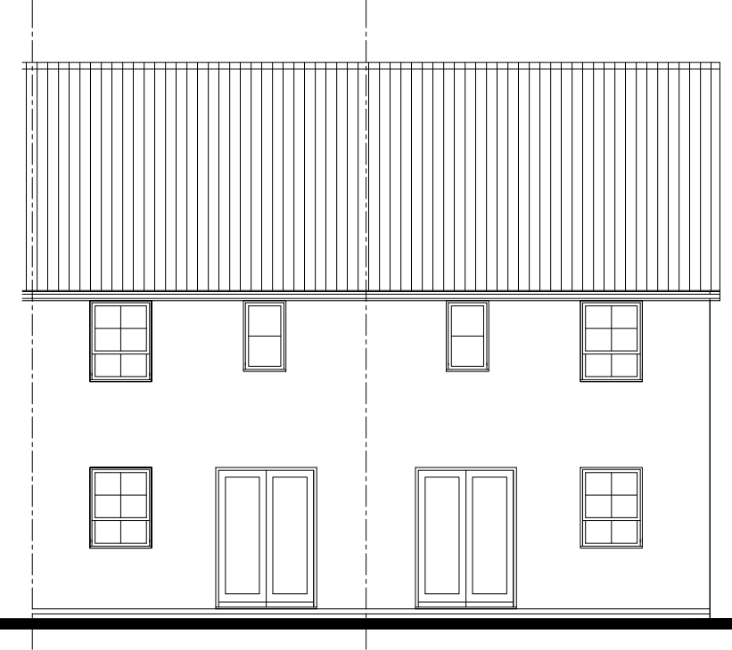
REAR ELEVATION
