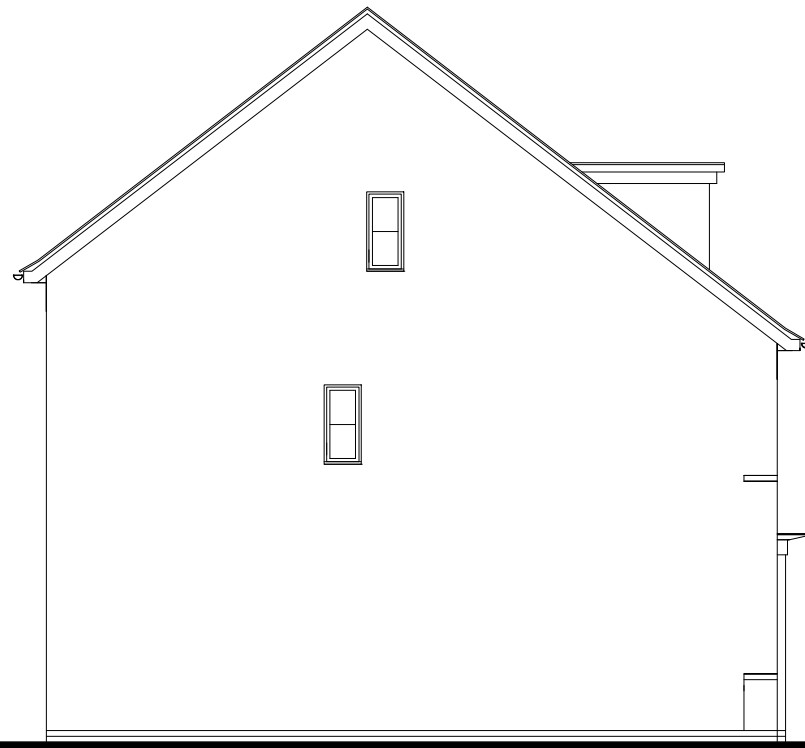
SIDE ELEVATION
