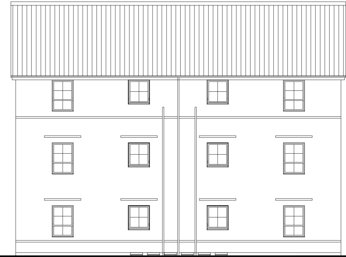
Rear Elevation
