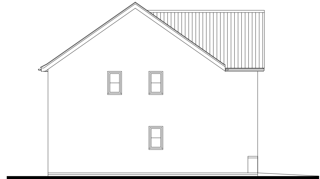
SIDE ELEVATION
