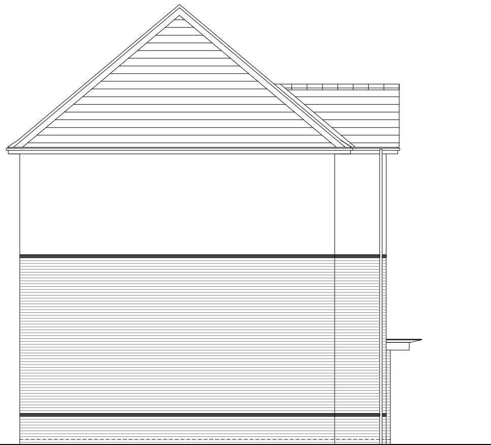
SIDE ELEVATION
